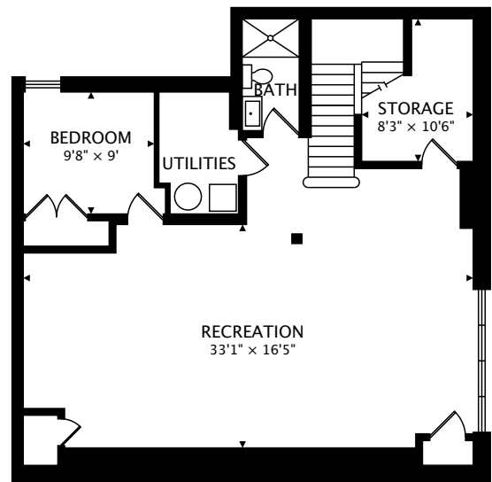
LOWER 1075 sq ft BELOW GRADE
