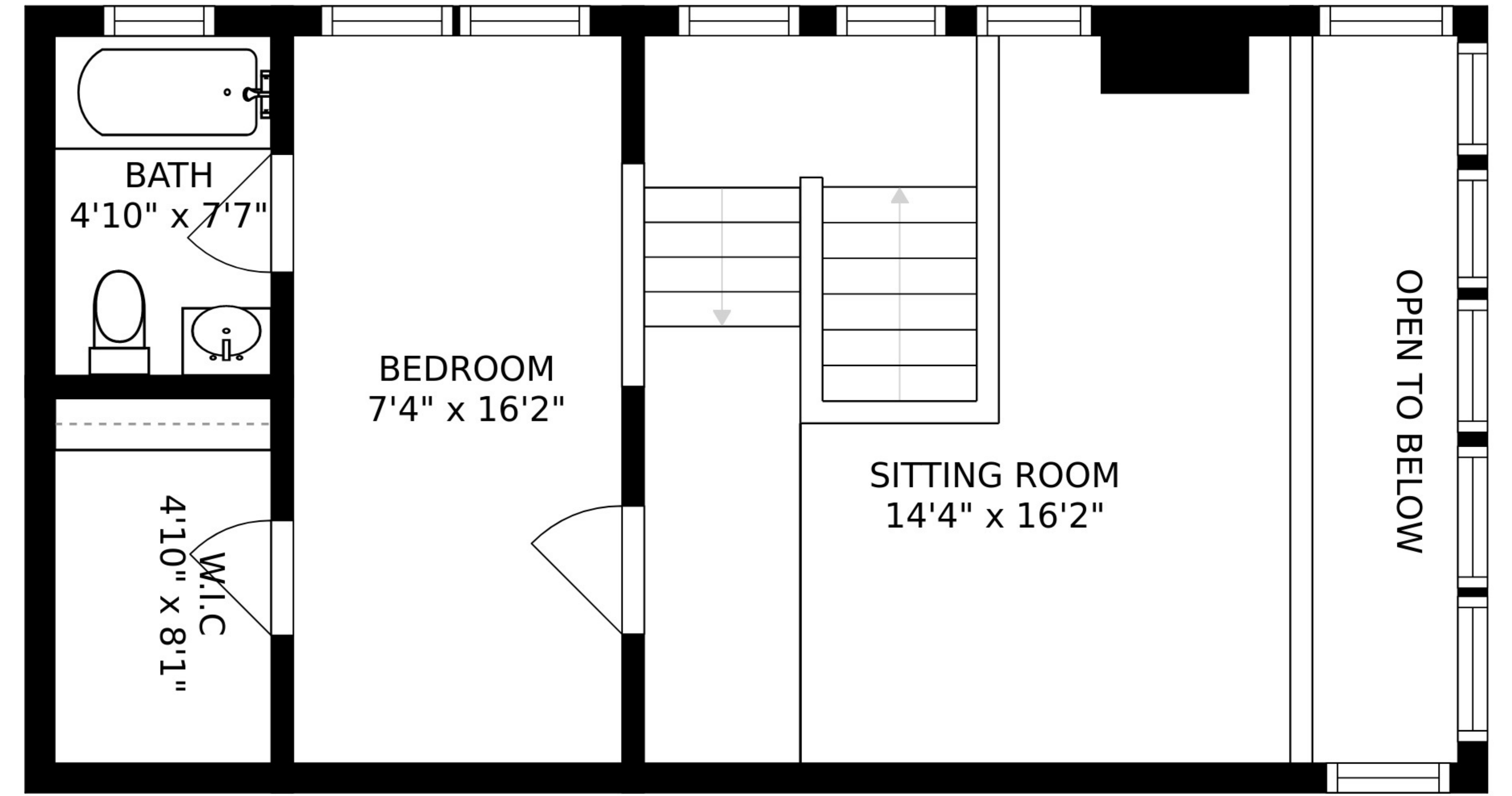
FLOOR 2
