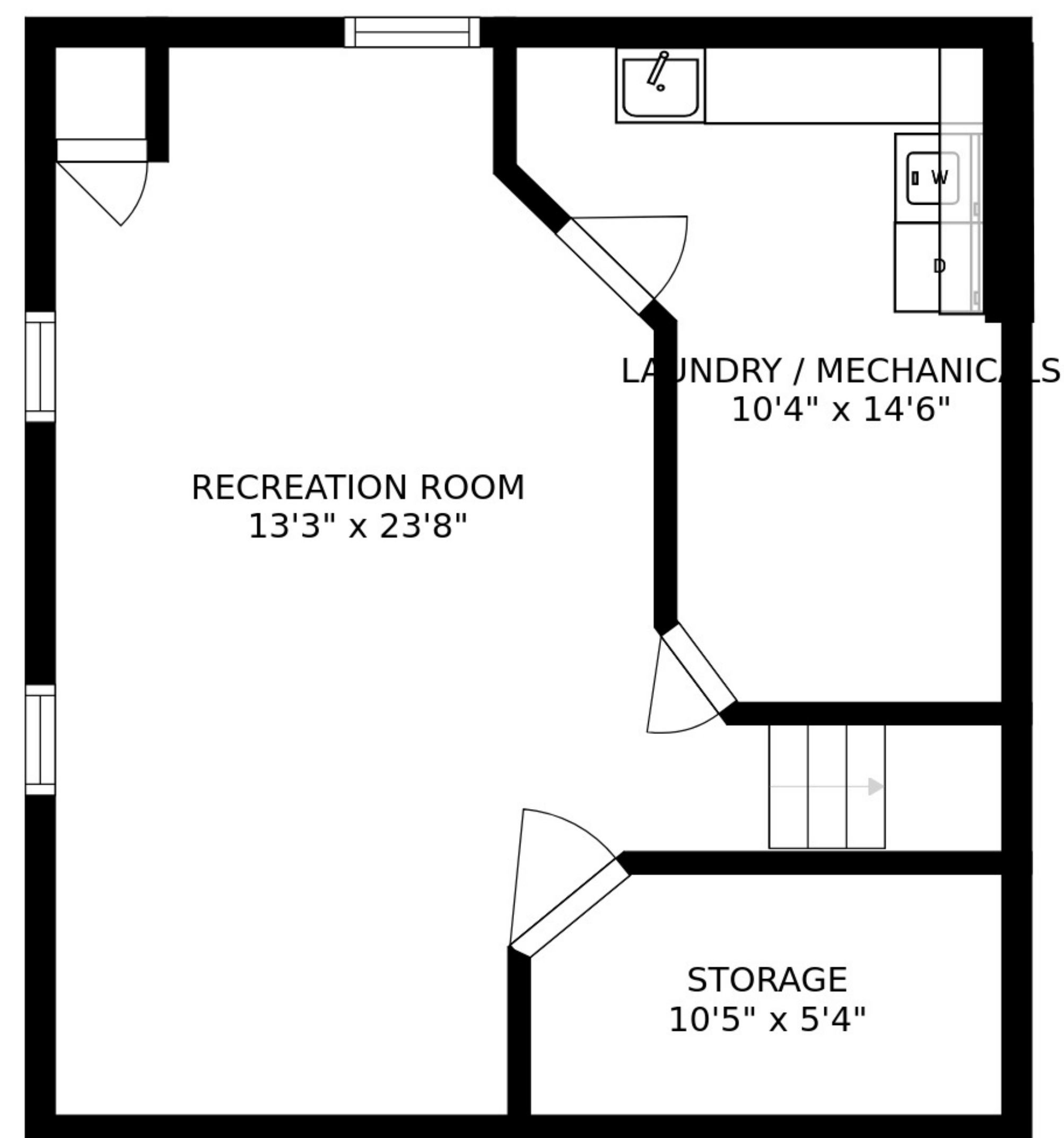
FLOOR 1
