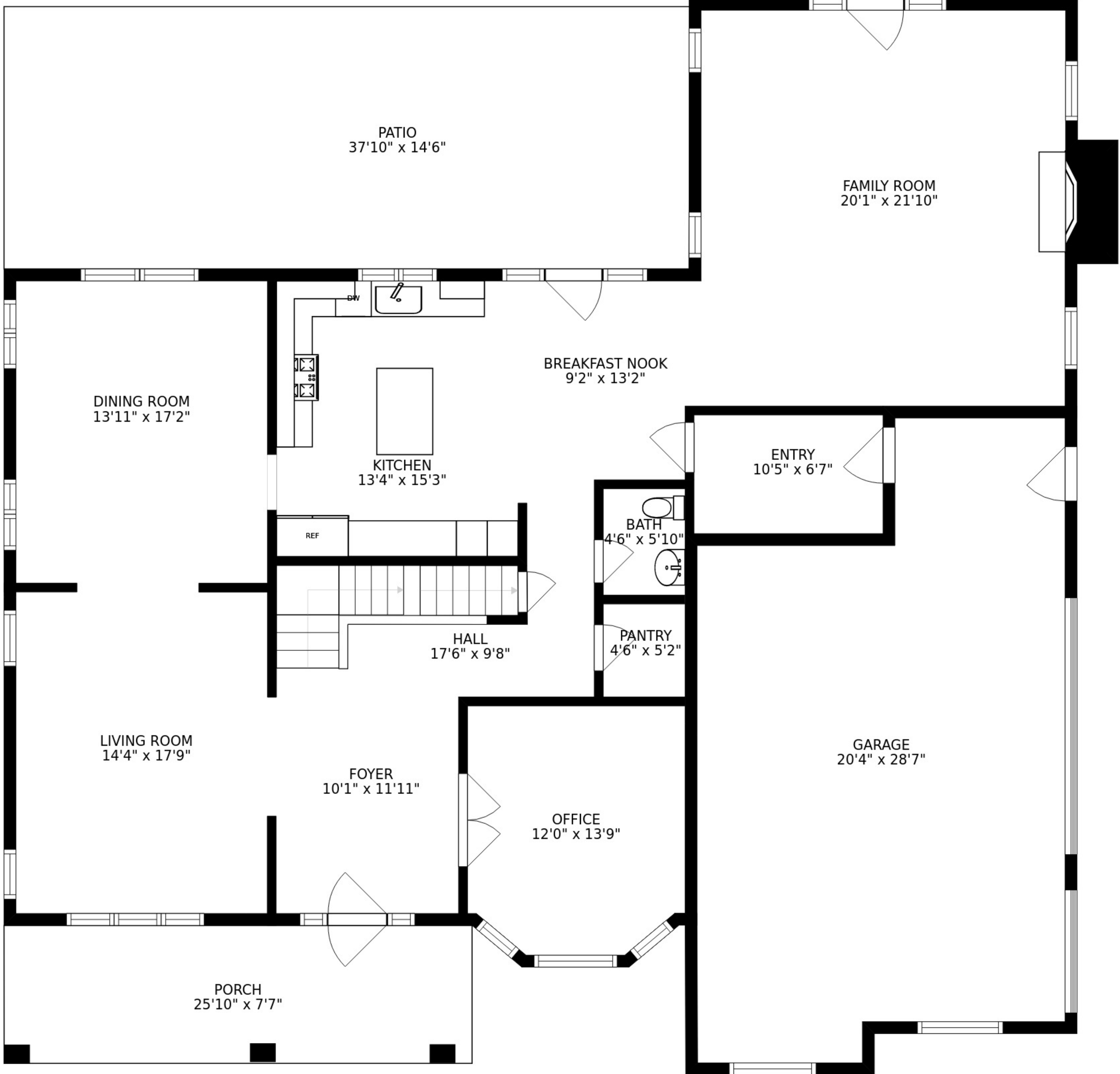
FLOOR 2
