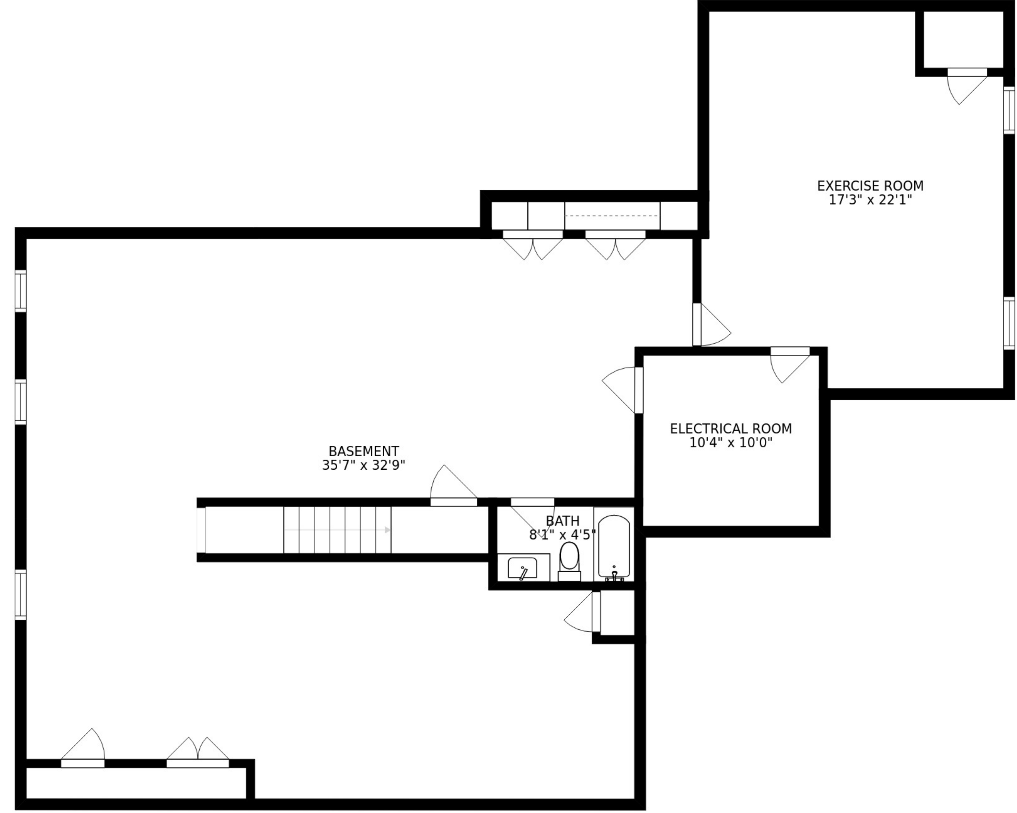
FLOOR 1
