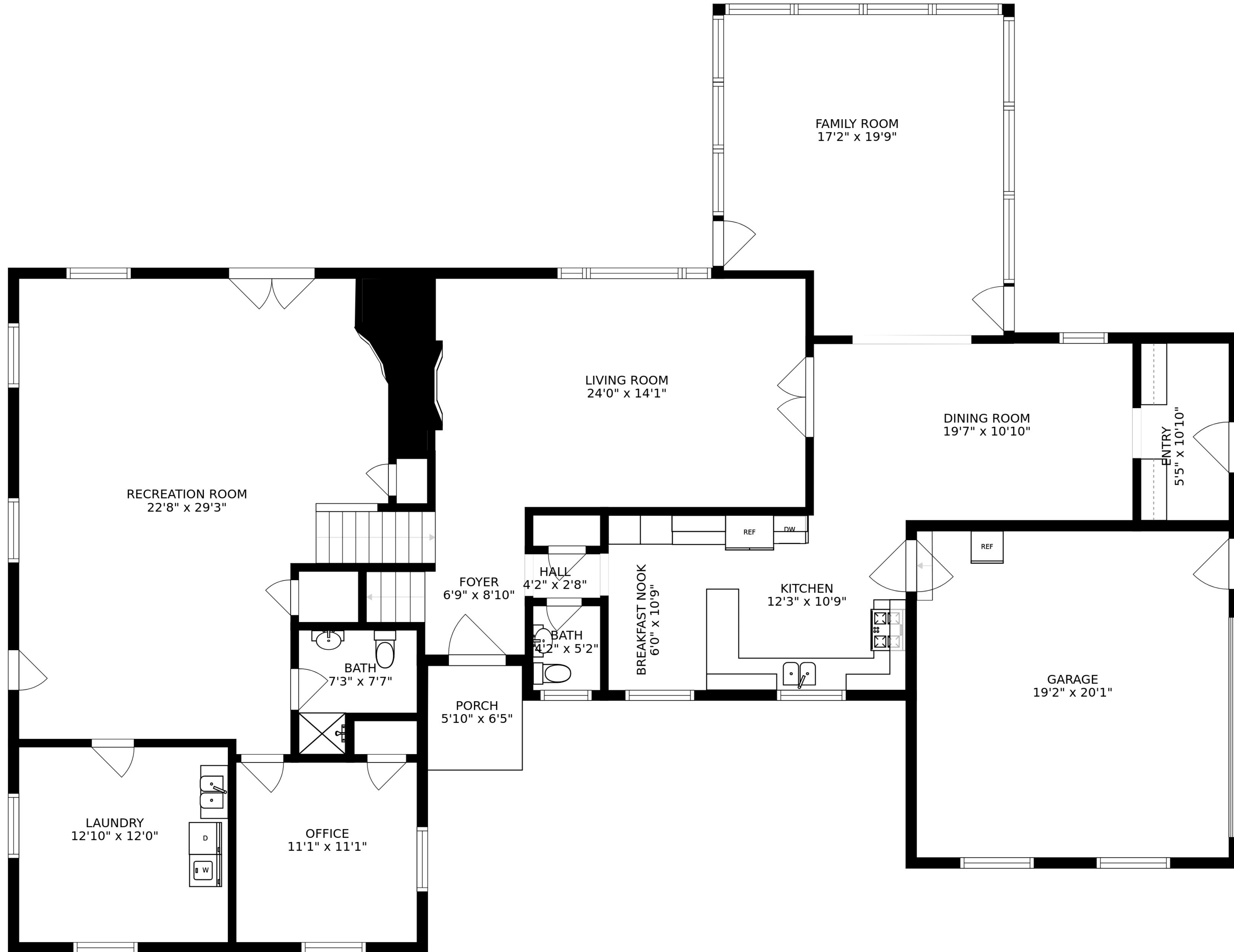
FLOOR 1
