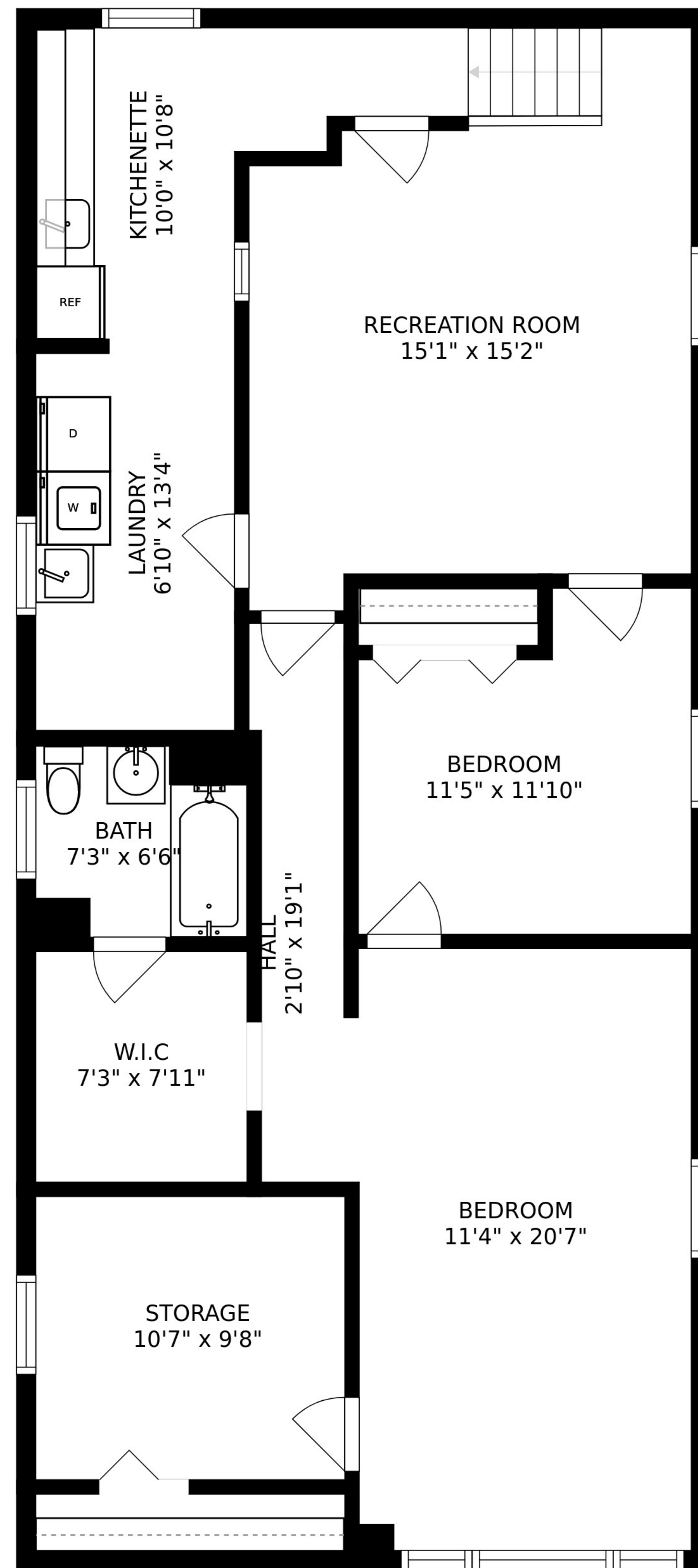
FLOOR 1
