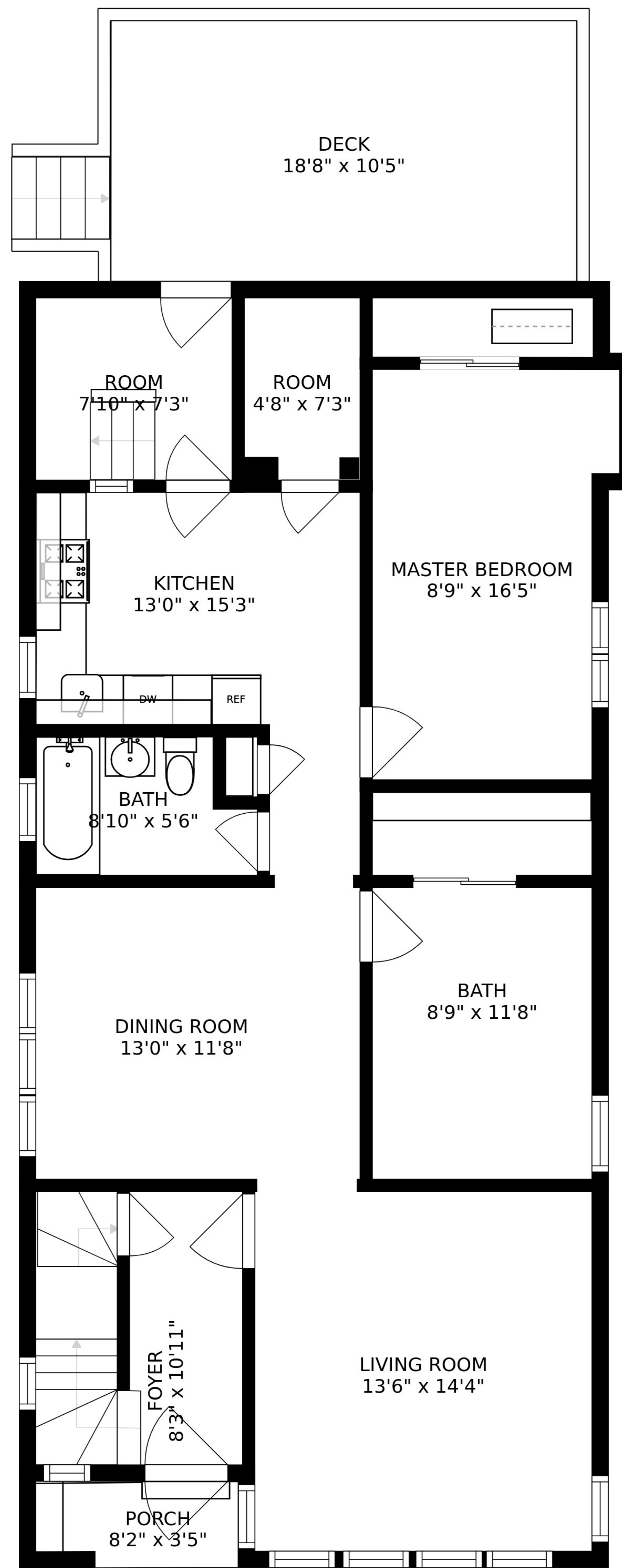
FLOOR 2
