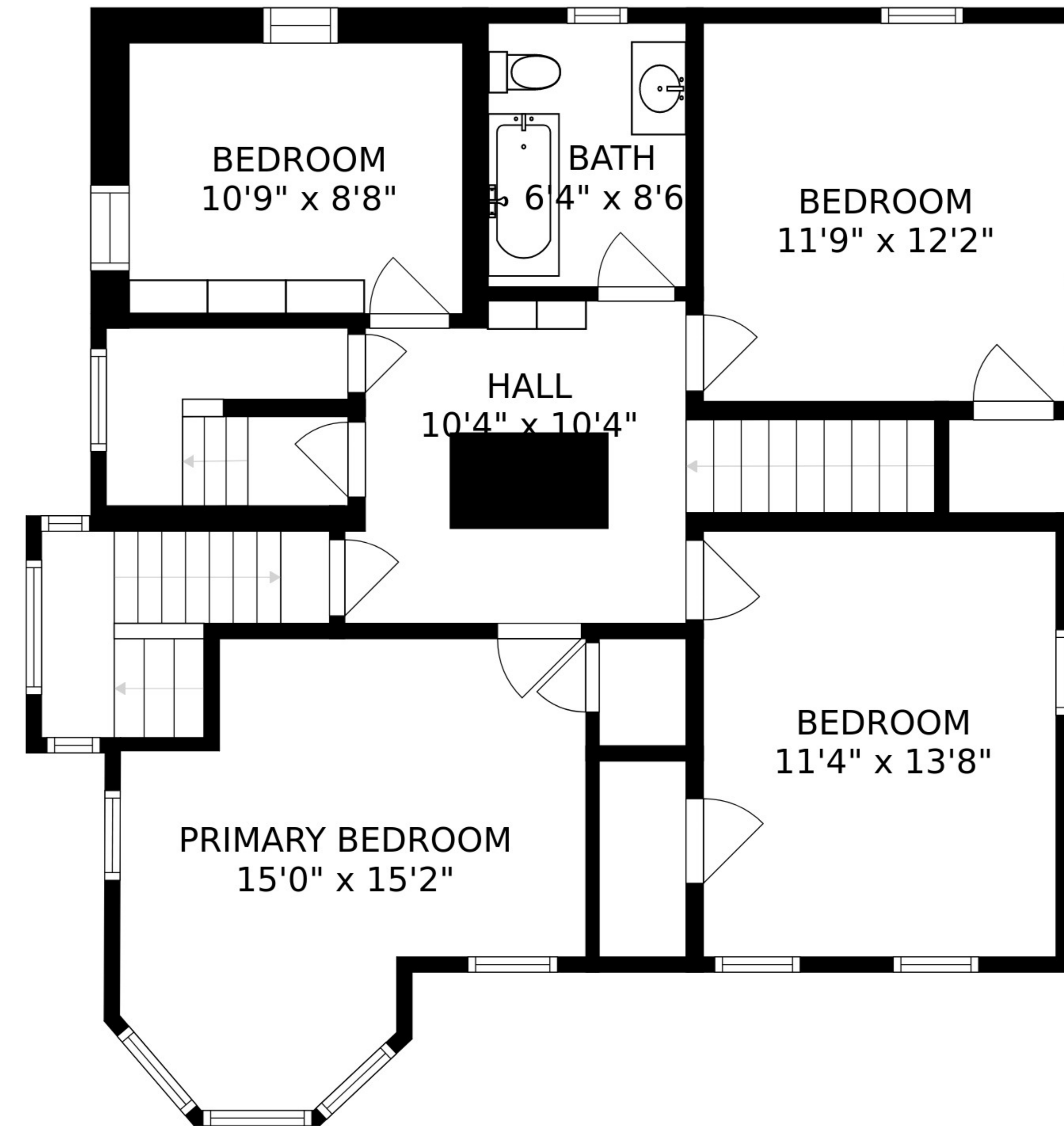
FLOOR 3
