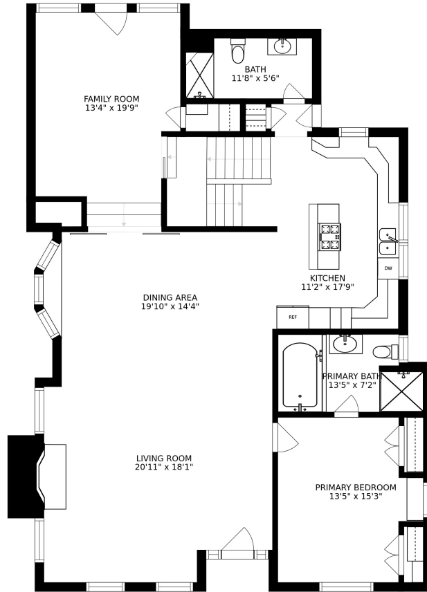
FLOOR 2
