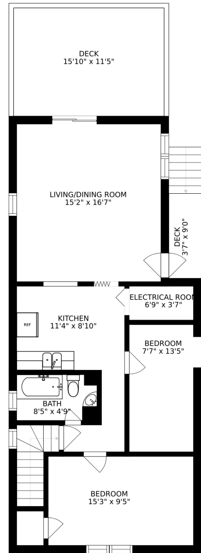
FLOOR 2
