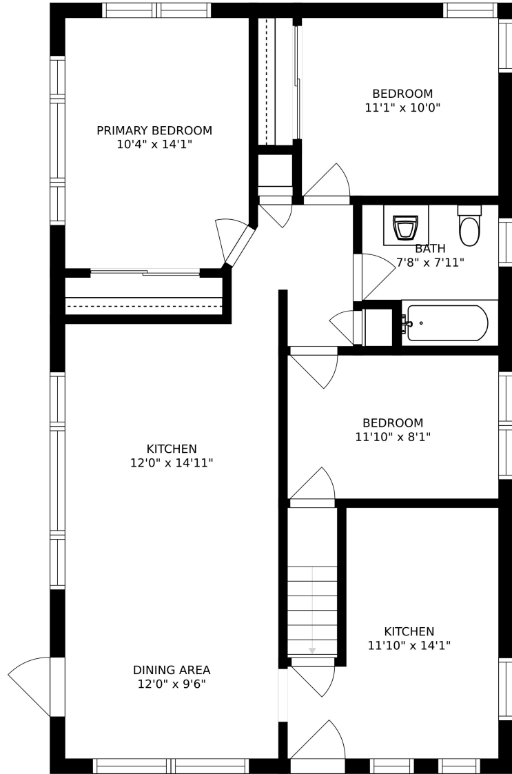
FLOOR 2
