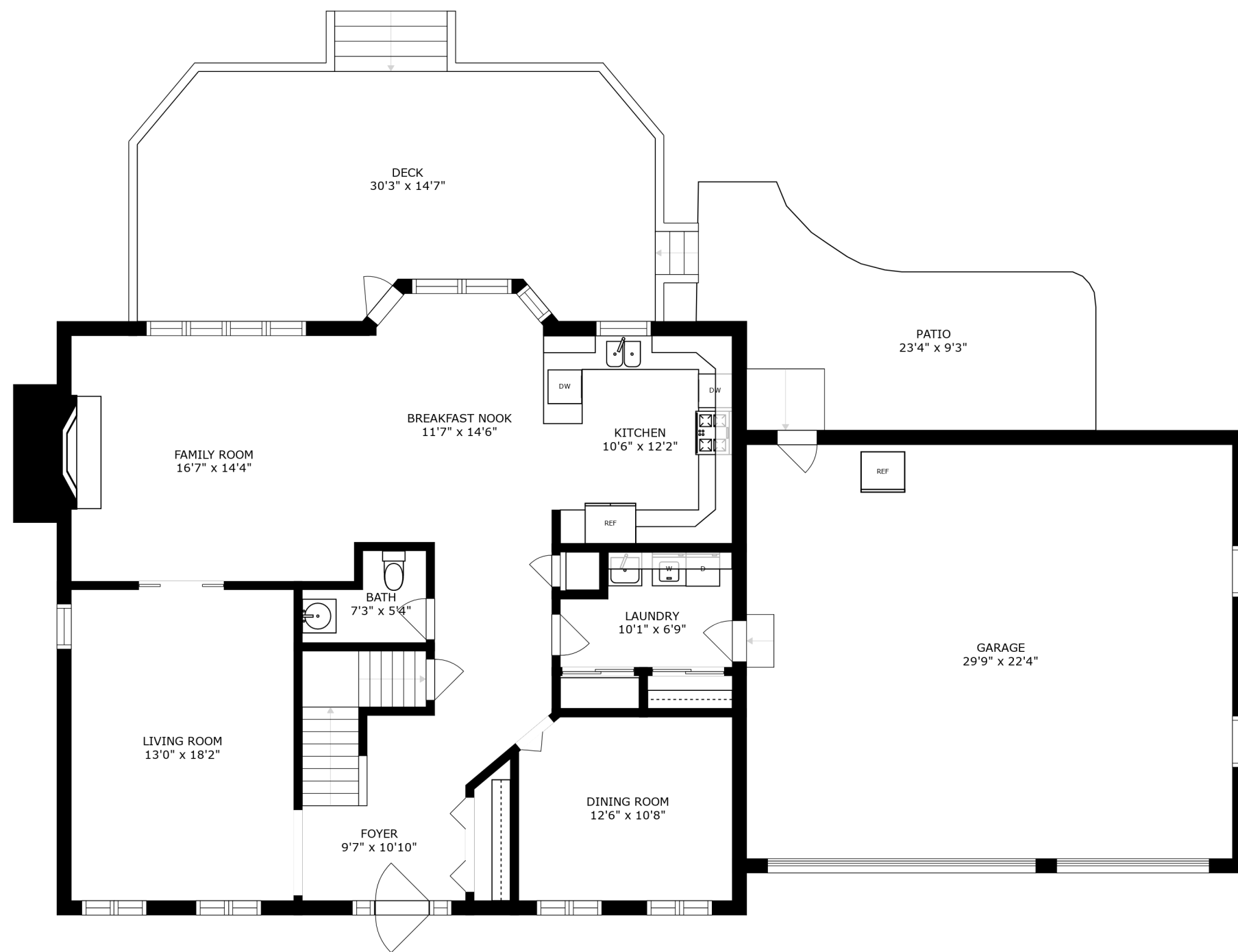
FLOOR 2
