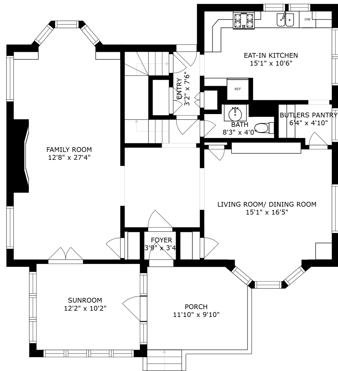
FLOOR 2
