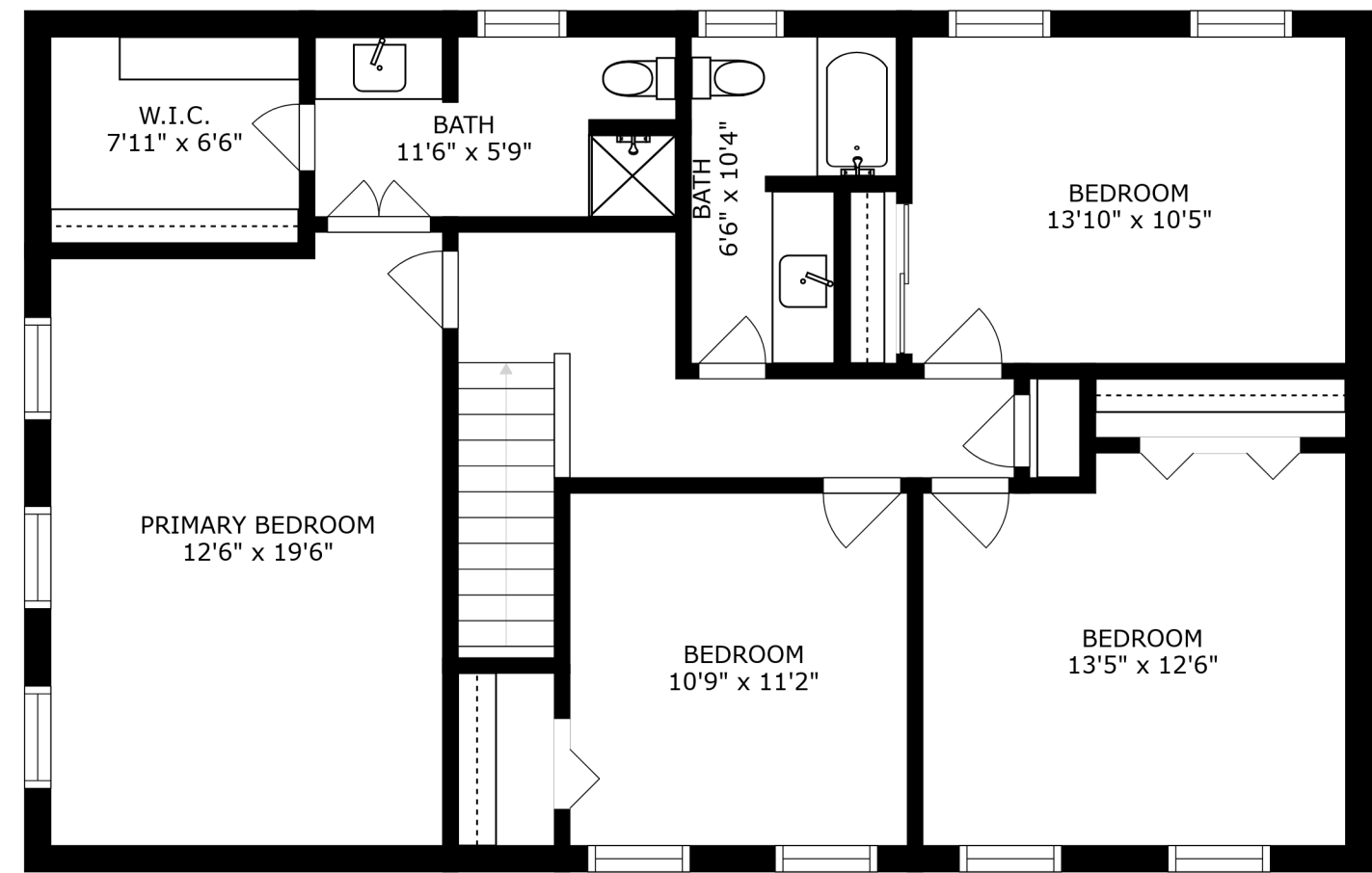
FLOOR 3
