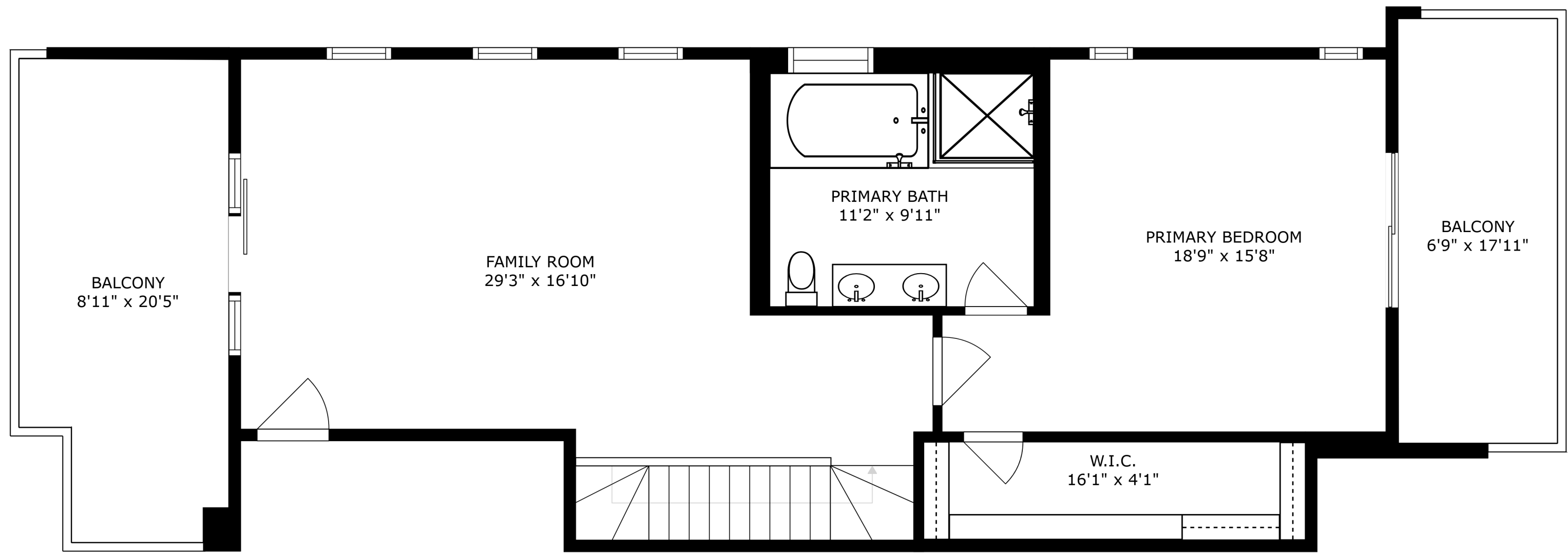
FLOOR 2
