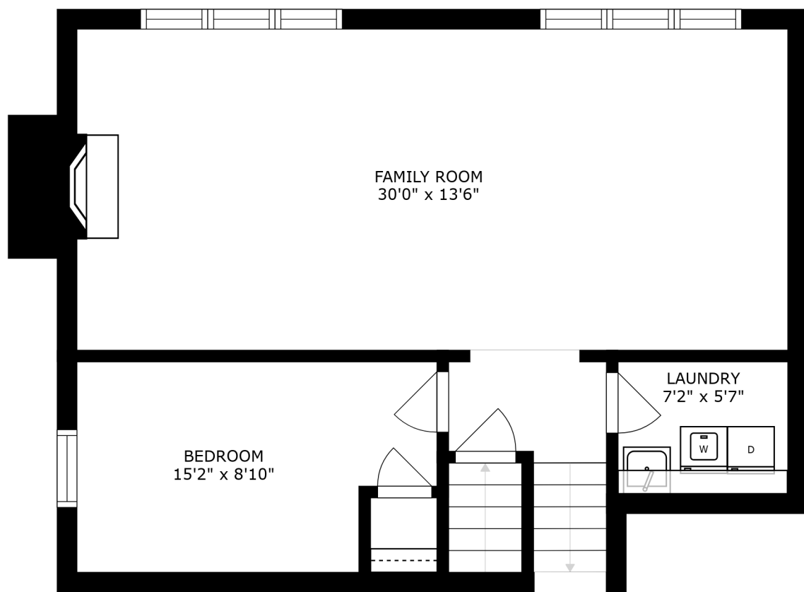
FLOOR 2
