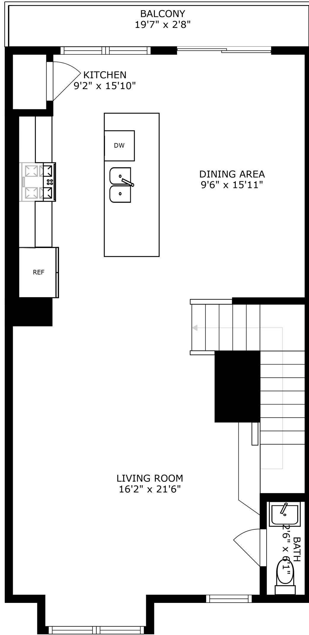
FLOOR 2
