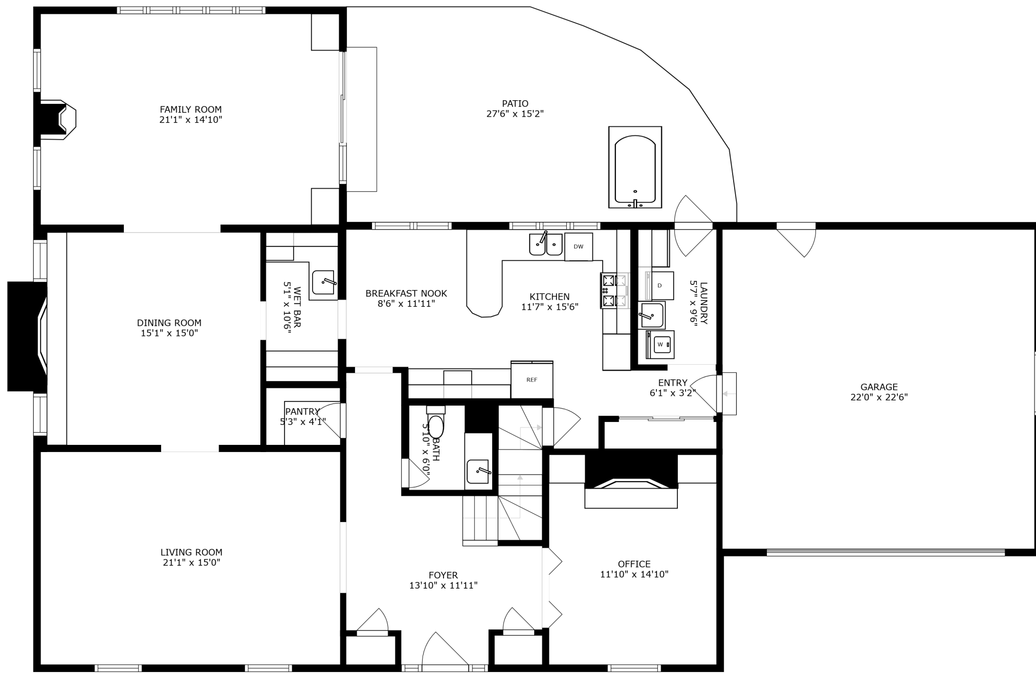
FLOOR 2
