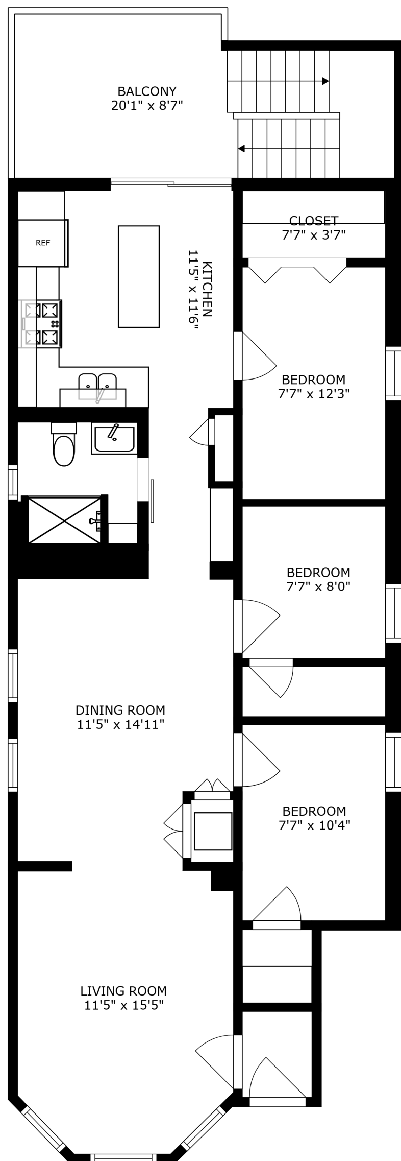
FLOOR 2
