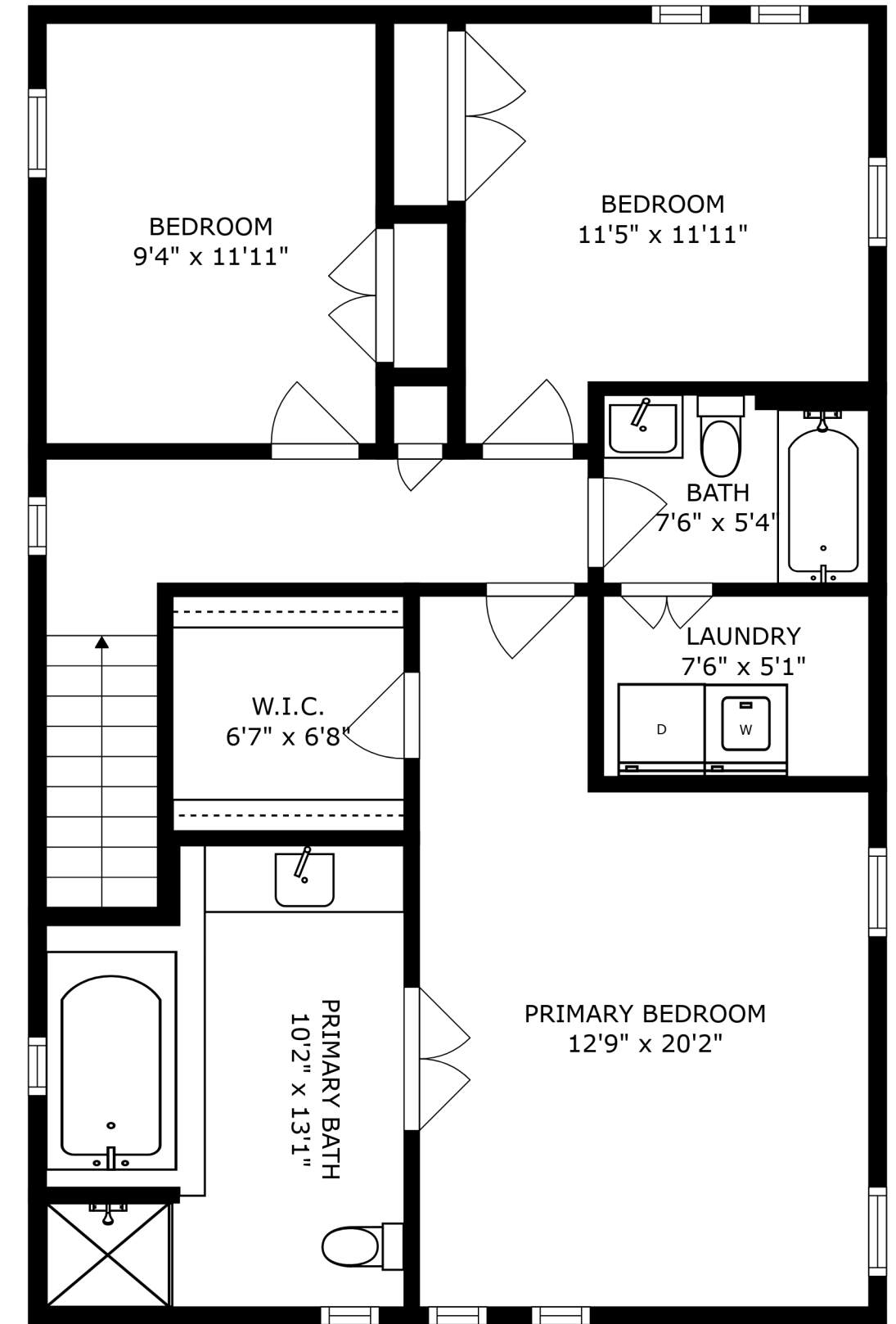
FLOOR 3
