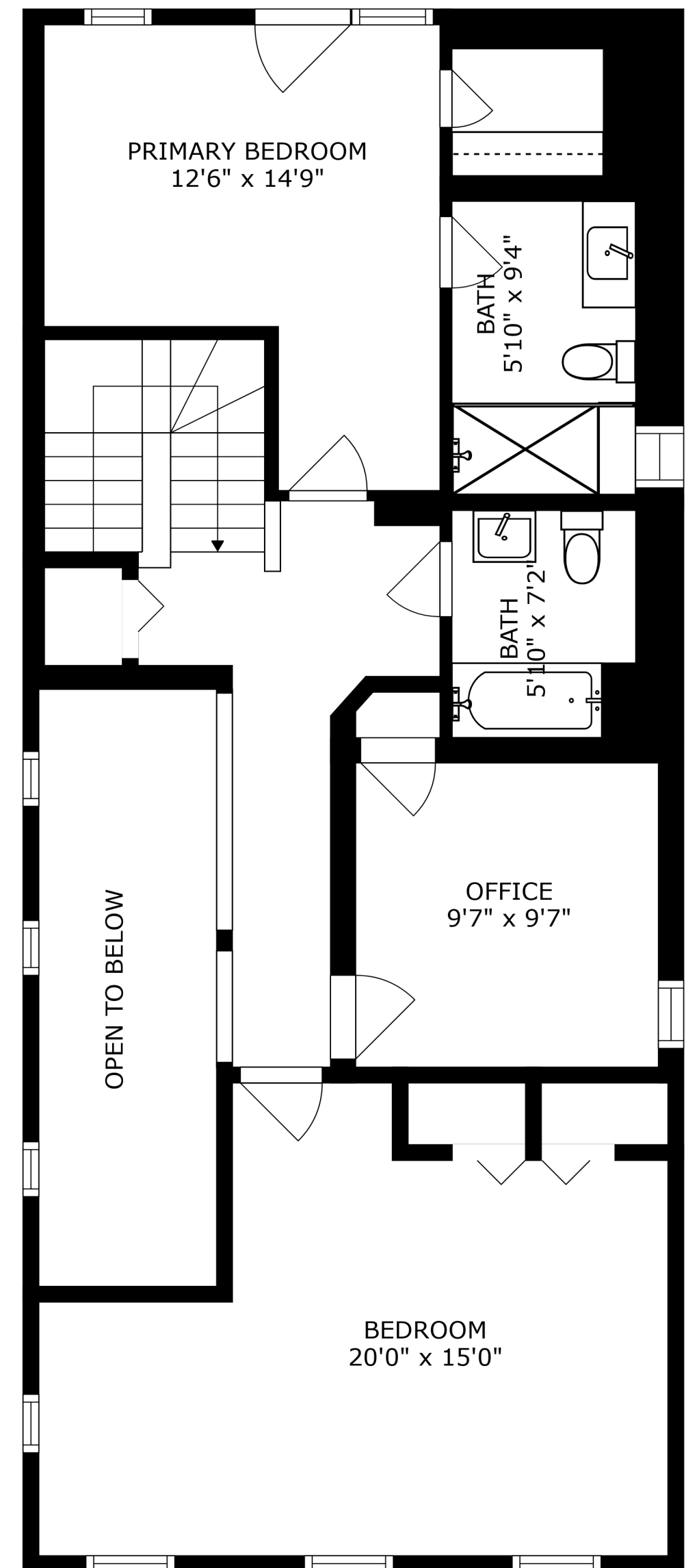
FLOOR 3
