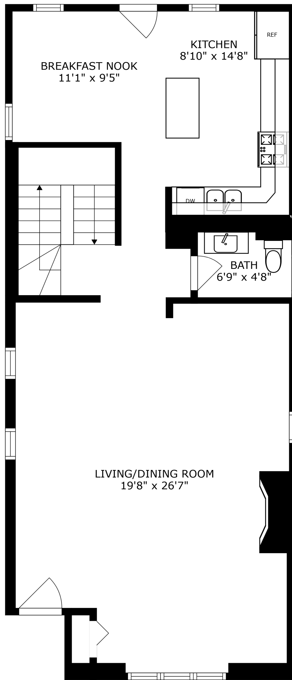
FLOOR 2
