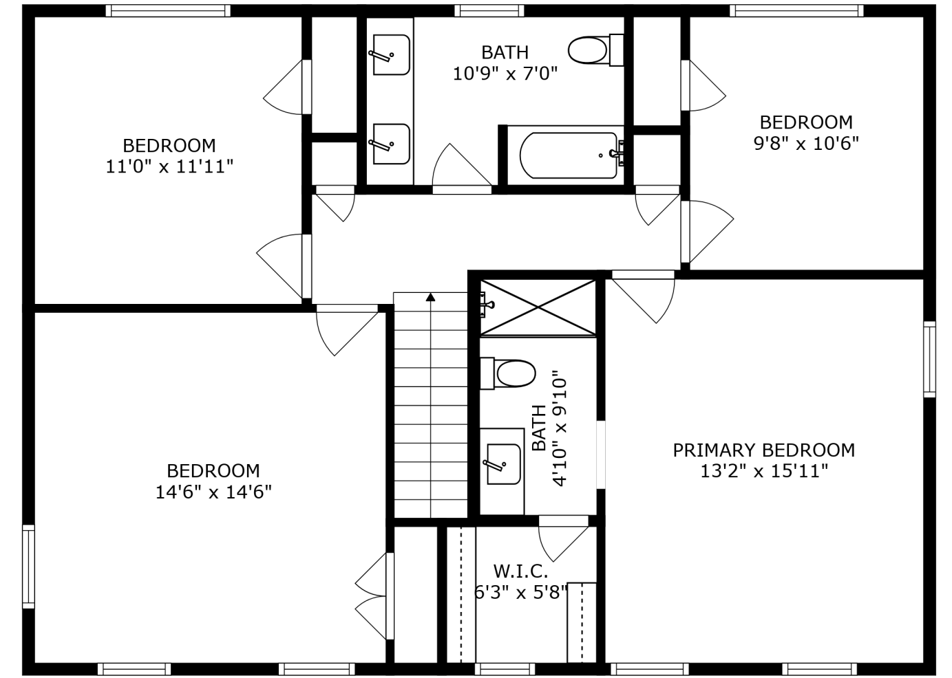
FLOOR 3
