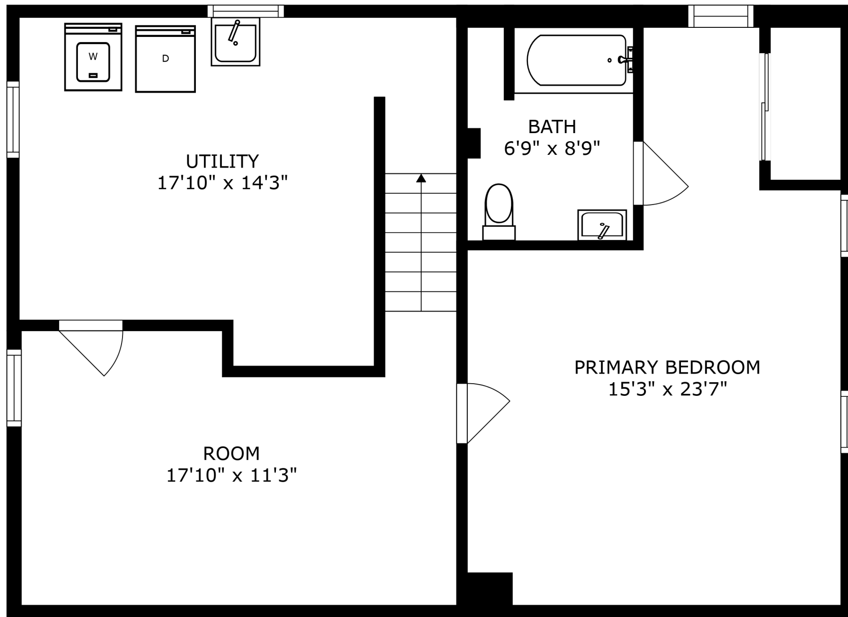
FLOOR 1
