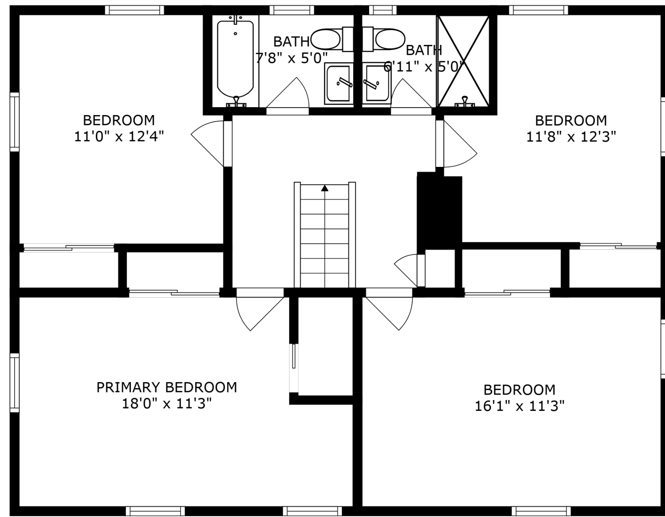
FLOOR 3
