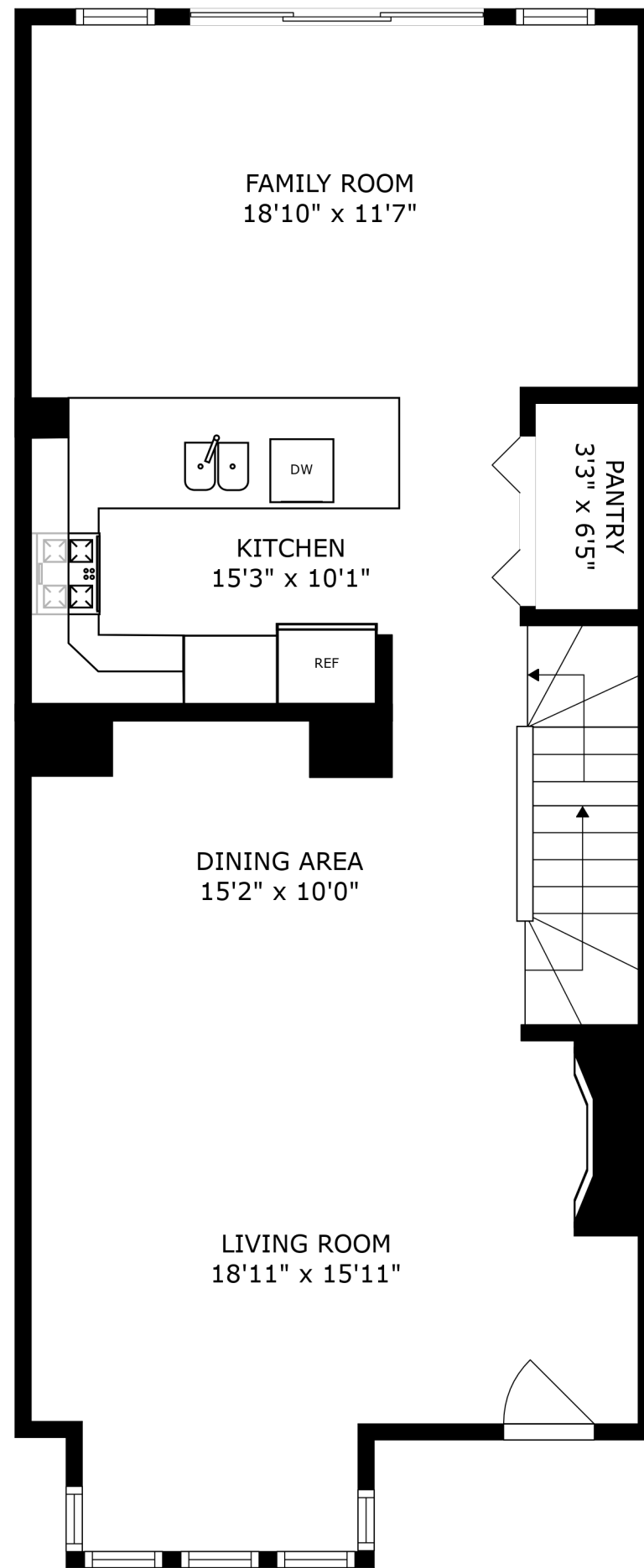
FLOOR 2
