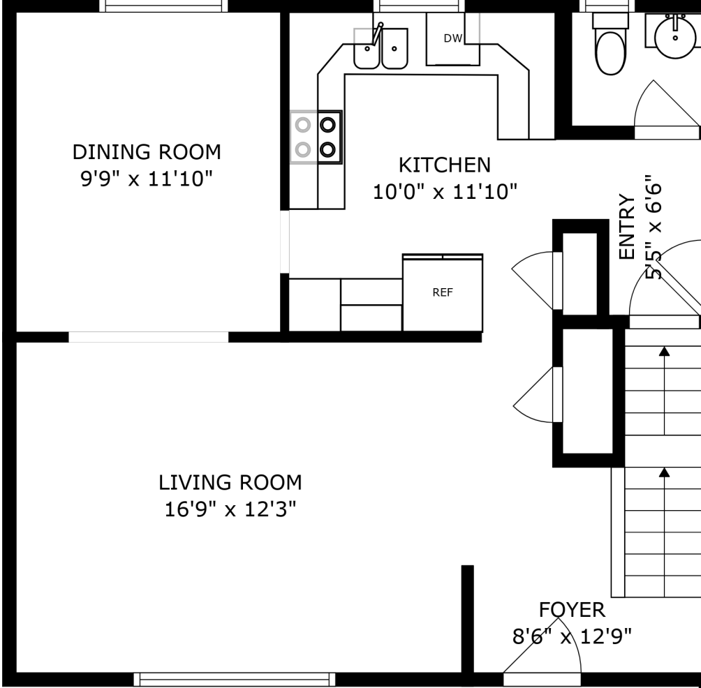
FLOOR 2
