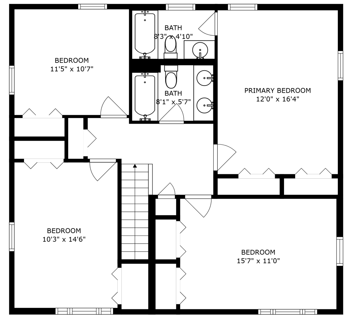
FLOOR 3
