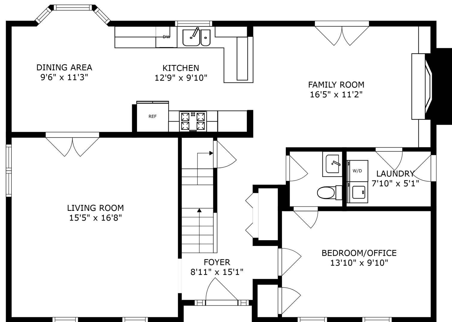
FLOOR 2
