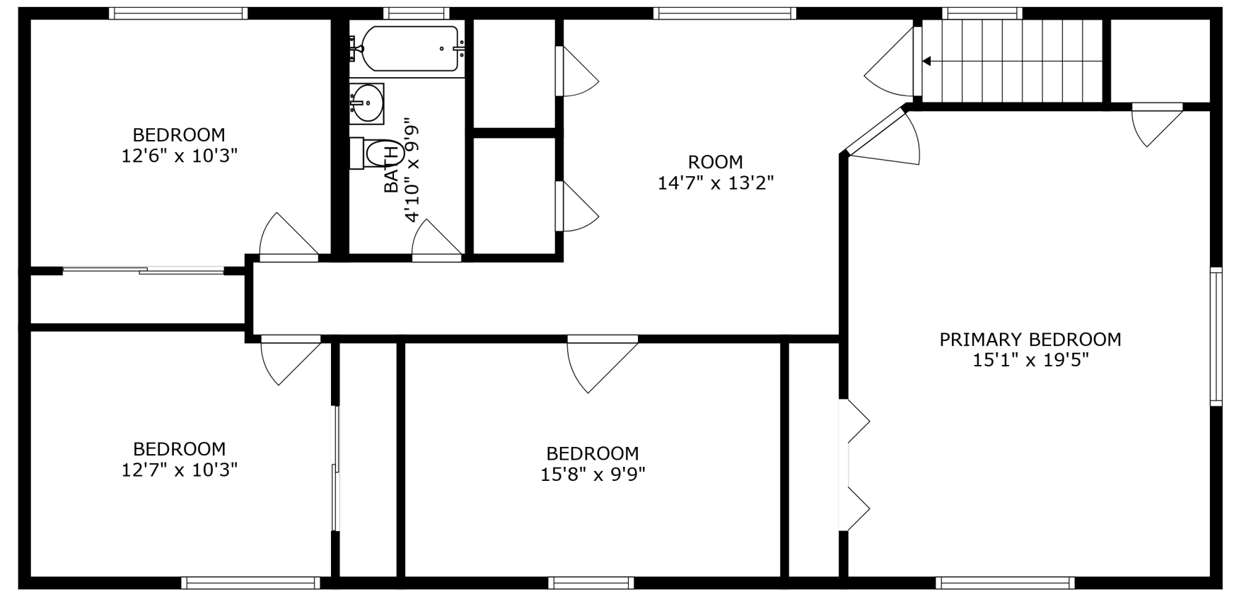
FLOOR 2
