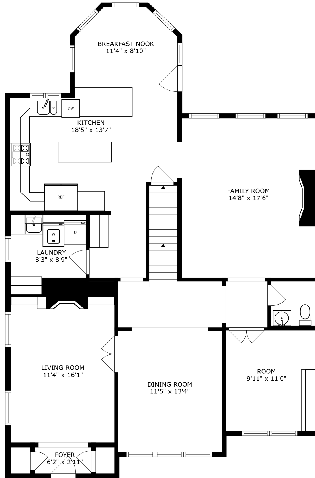
FLOOR 2
