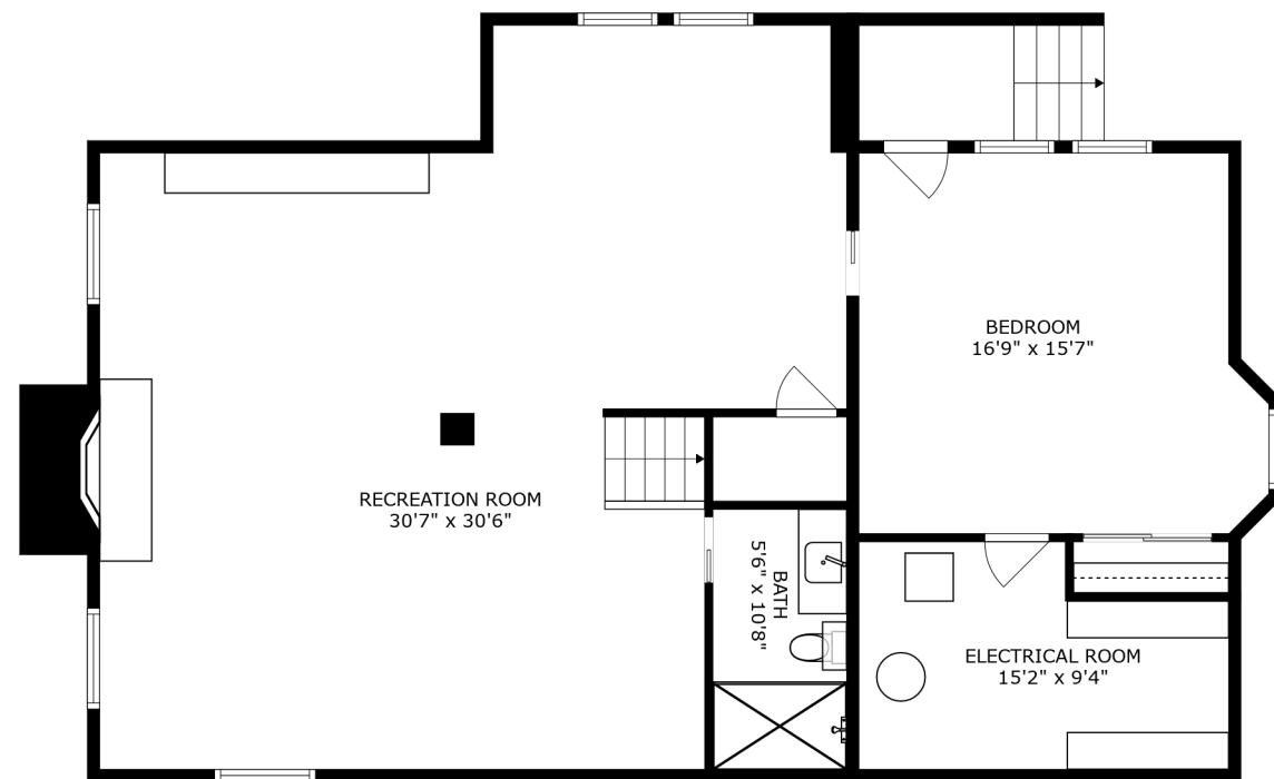
FLOOR 1
