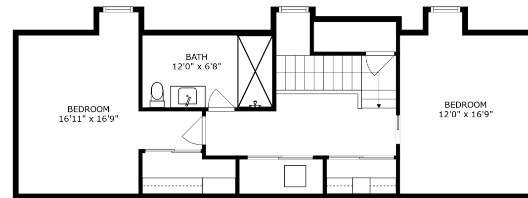
FLOOR 4
