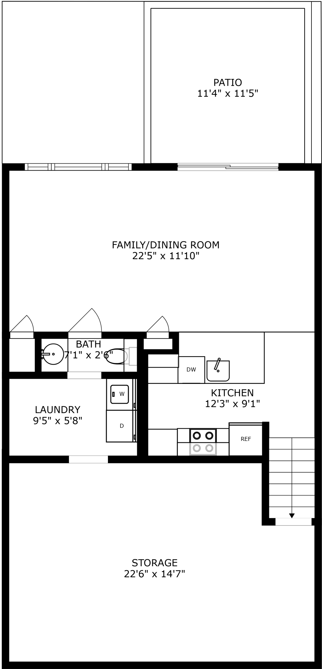
FLOOR 1
