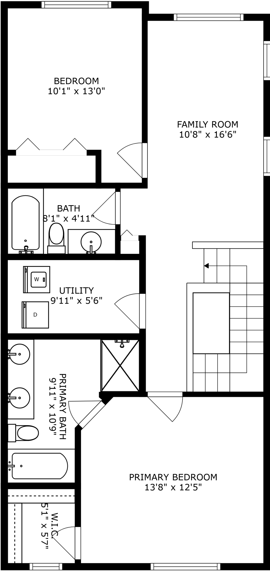
FLOOR 2
