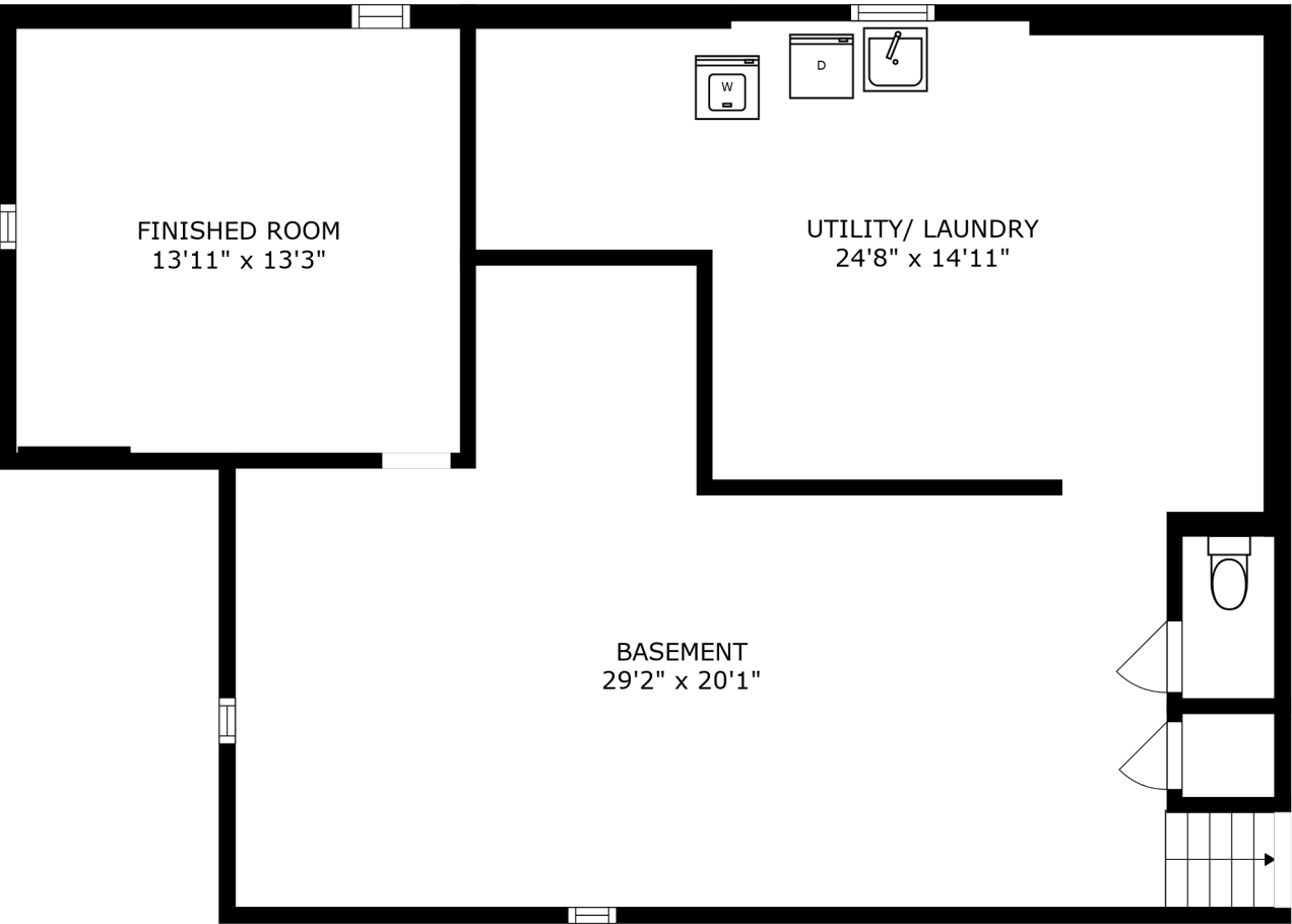
FLOOR 1
