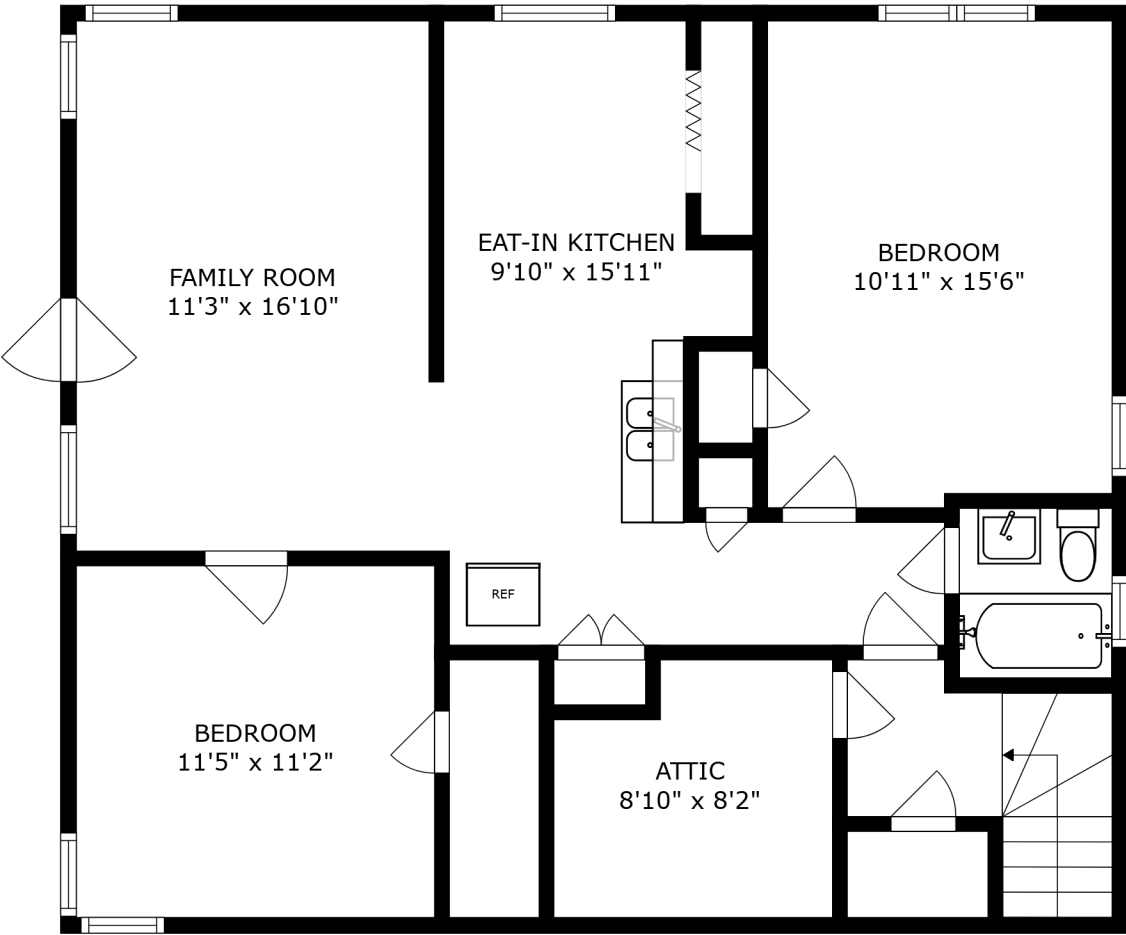
FLOOR 3
