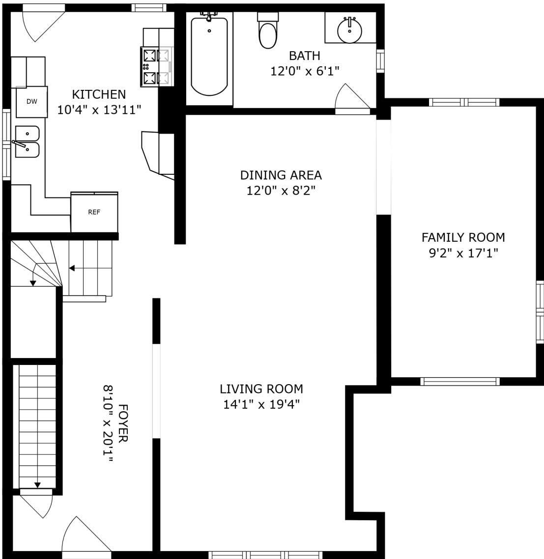
FLOOR 2
