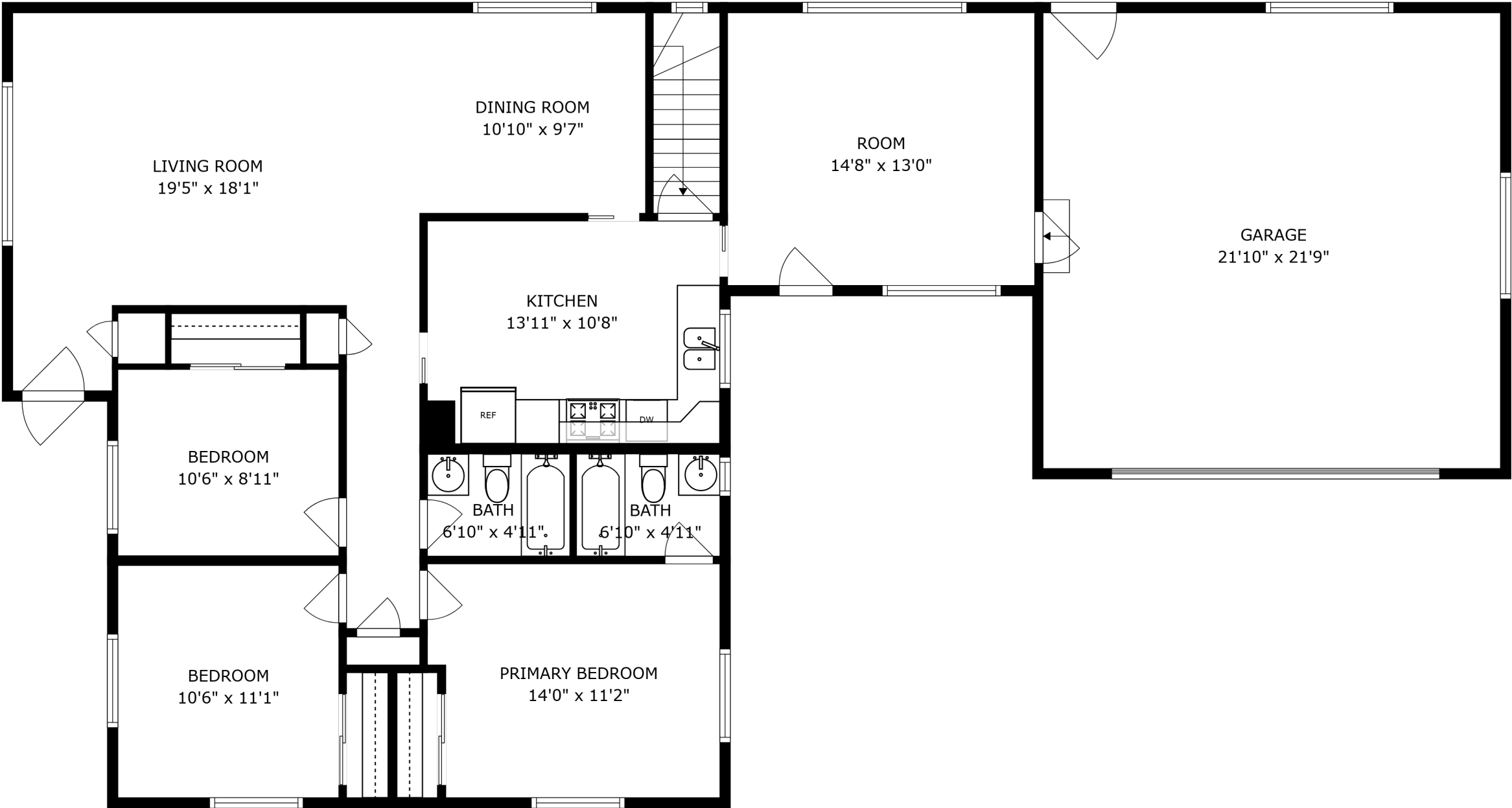
FLOOR 2
