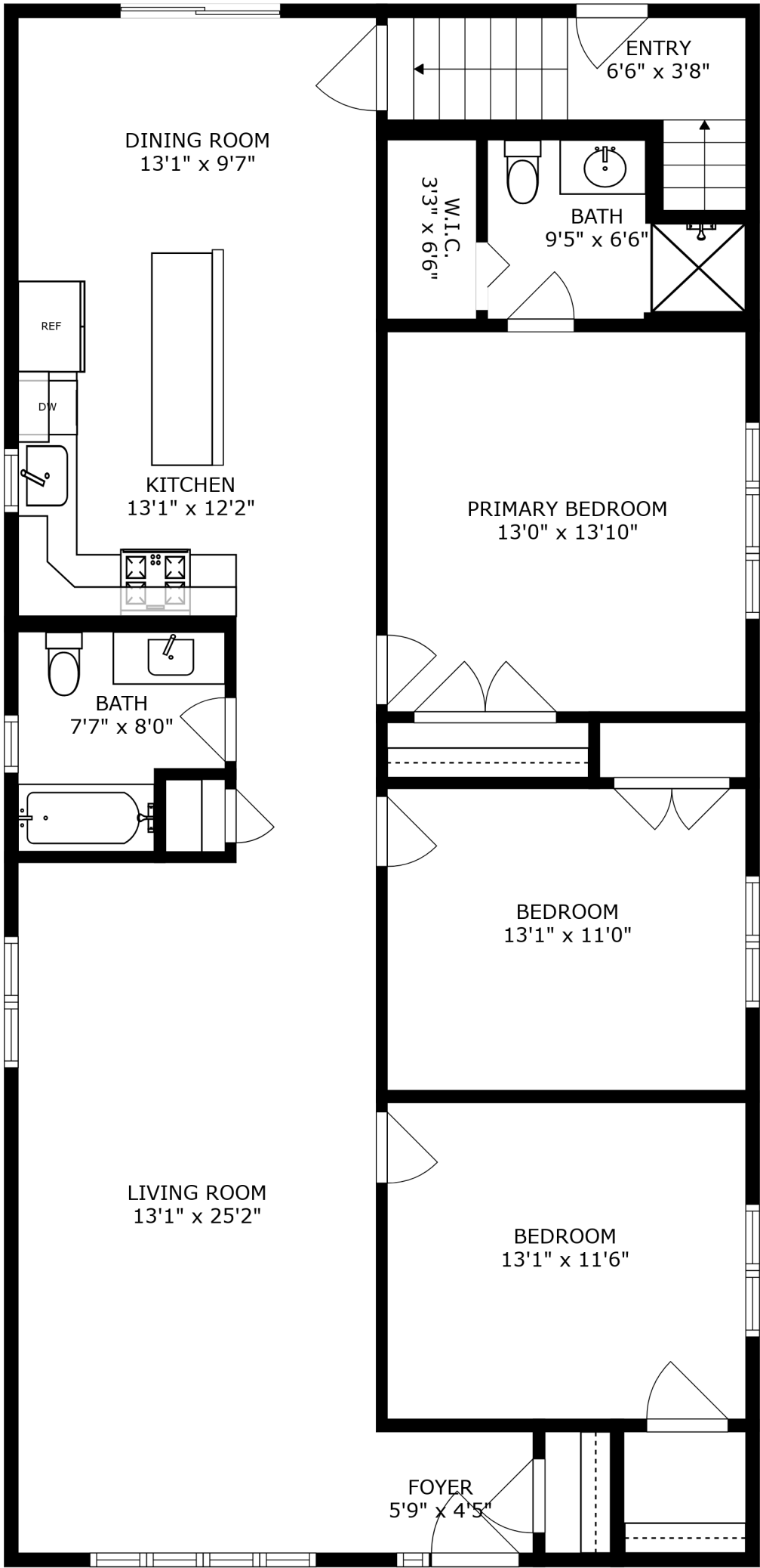
FLOOR 2
