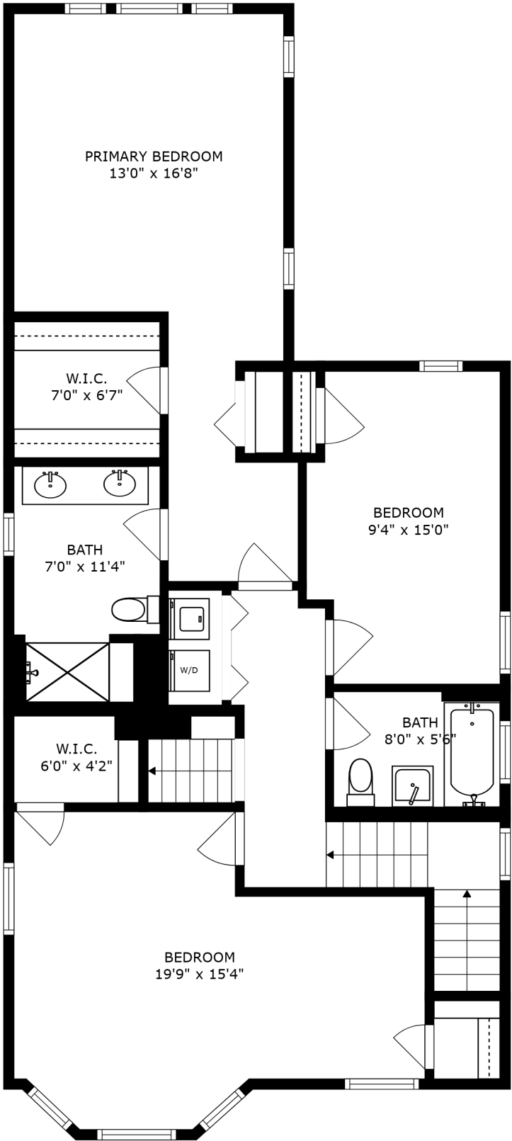
FLOOR 3
