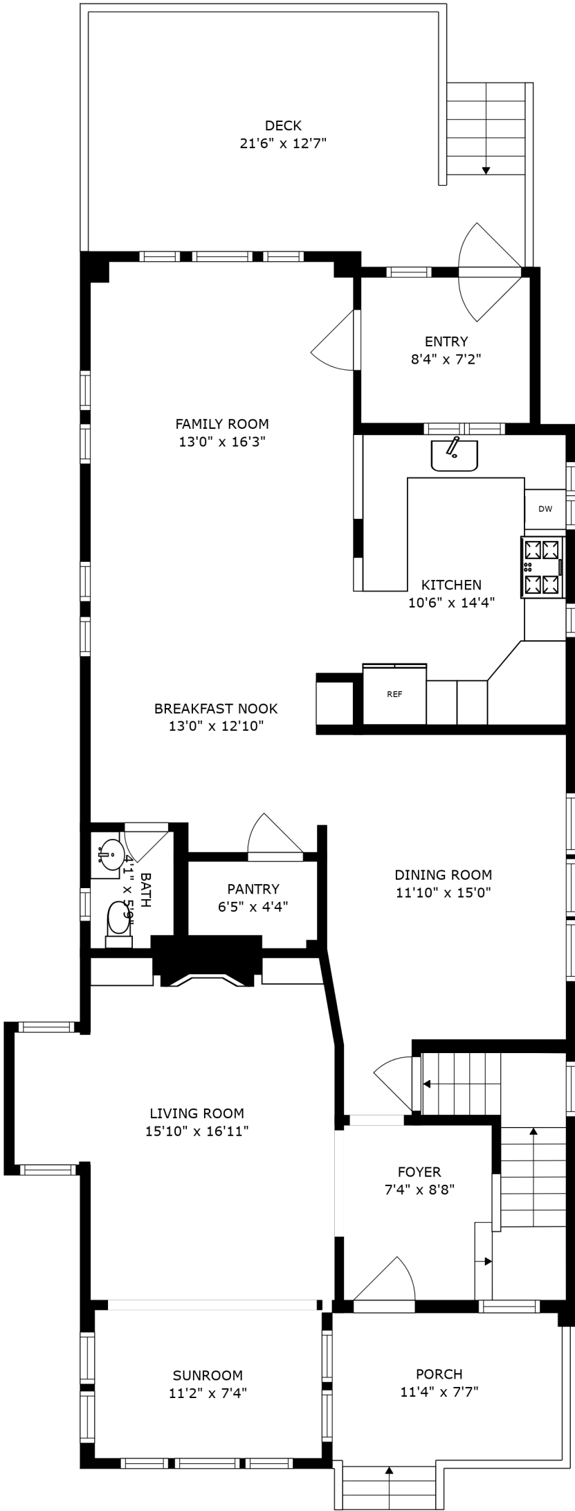
FLOOR 2
