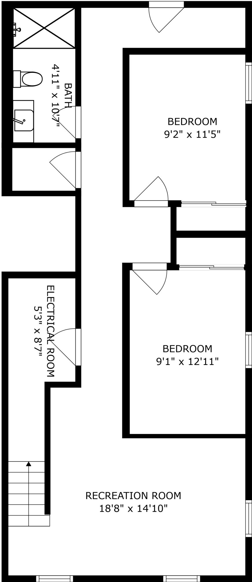
FLOOR 1
