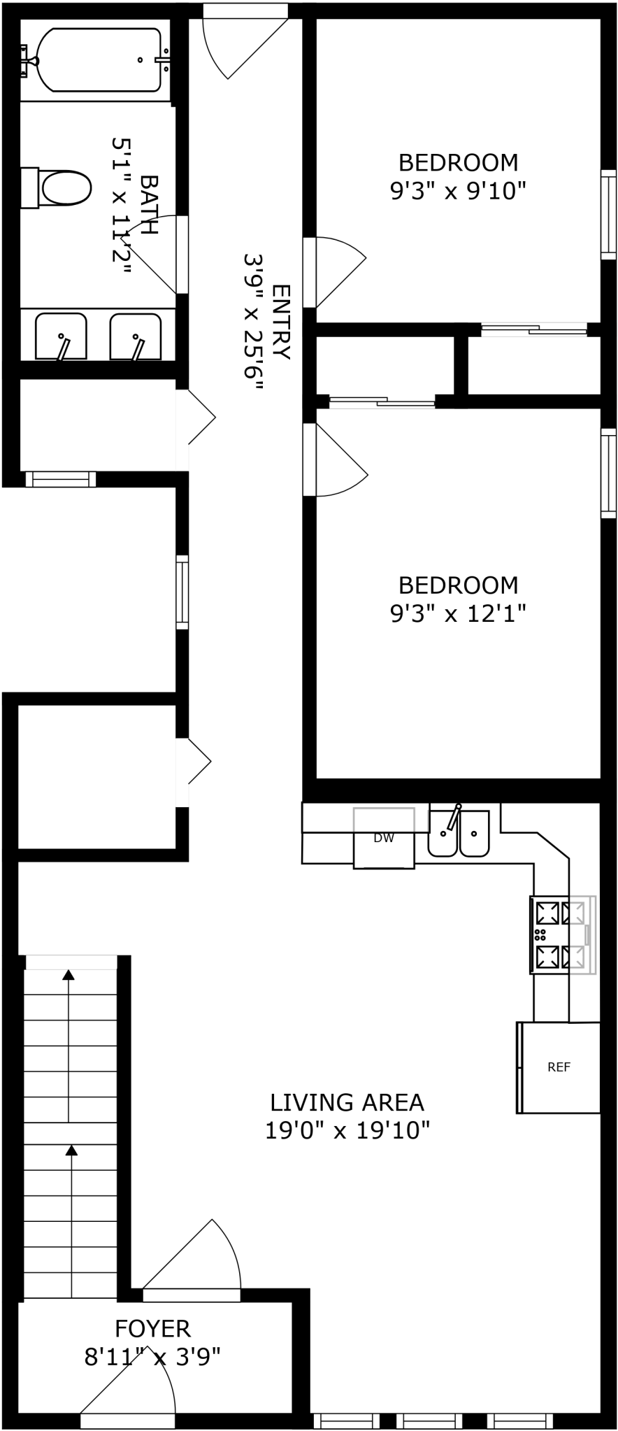
FLOOR 2
