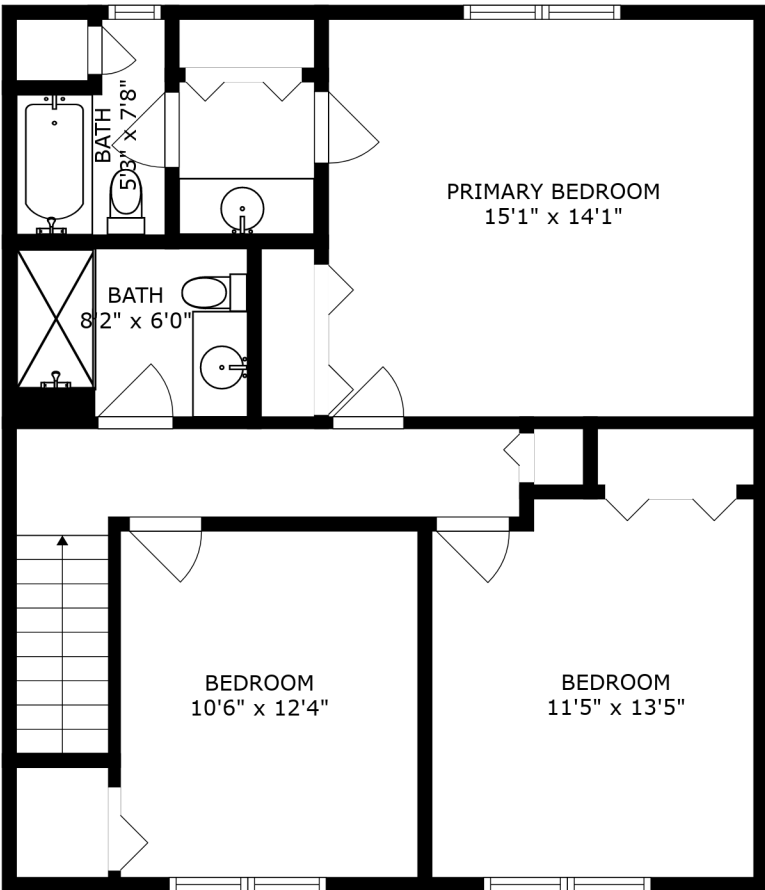
FLOOR 3
