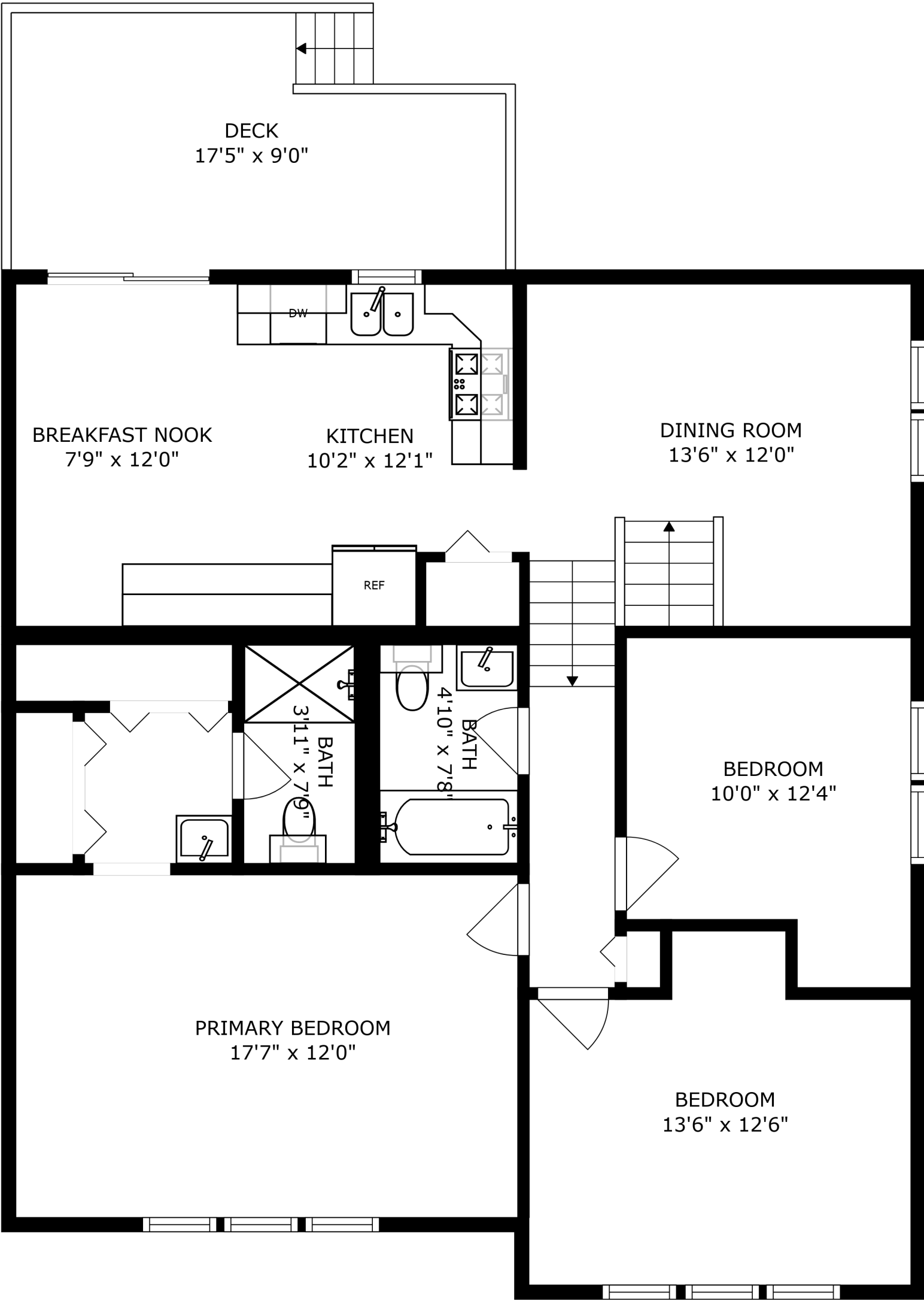
FLOOR 2
