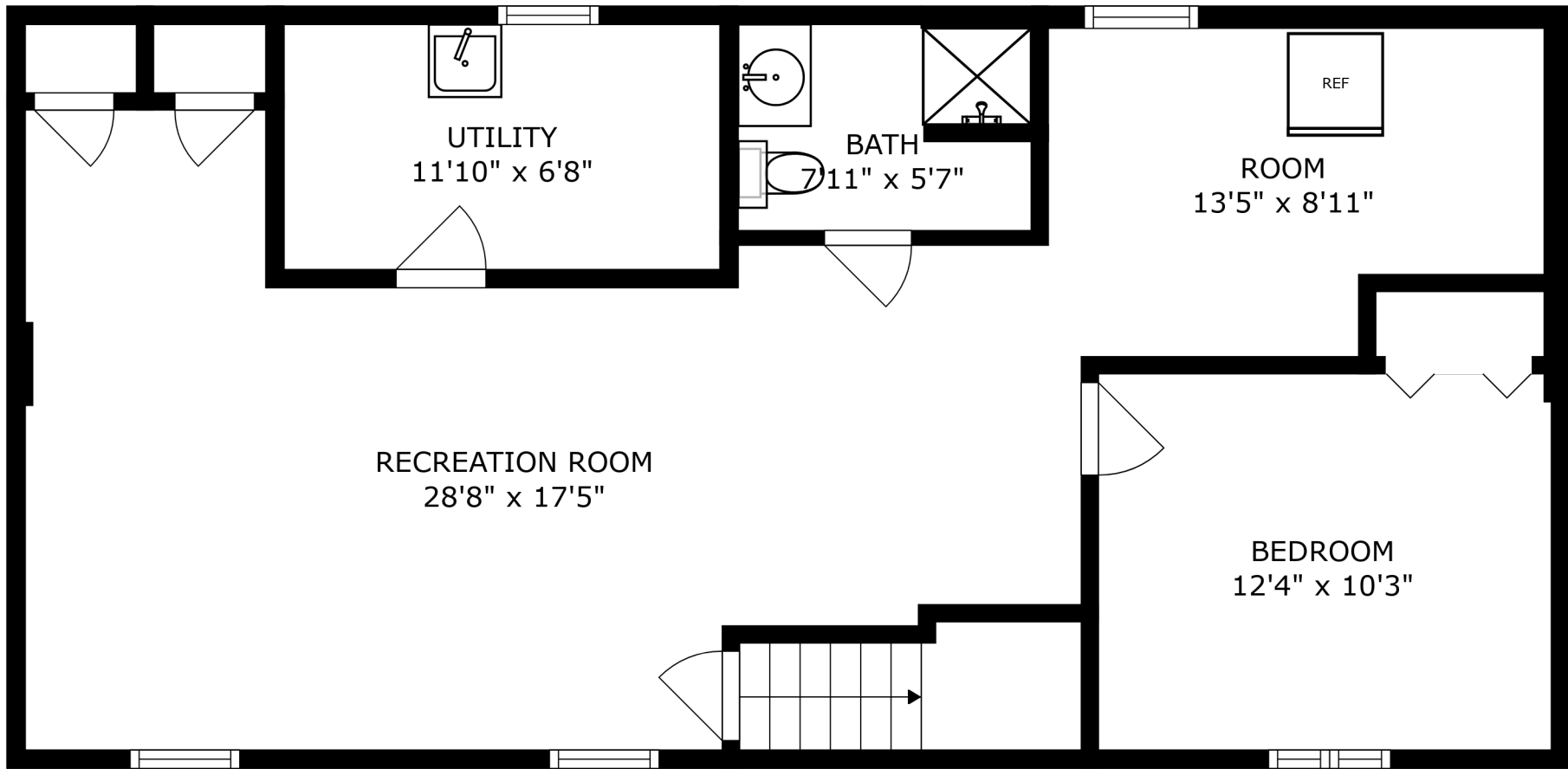
FLOOR 2
