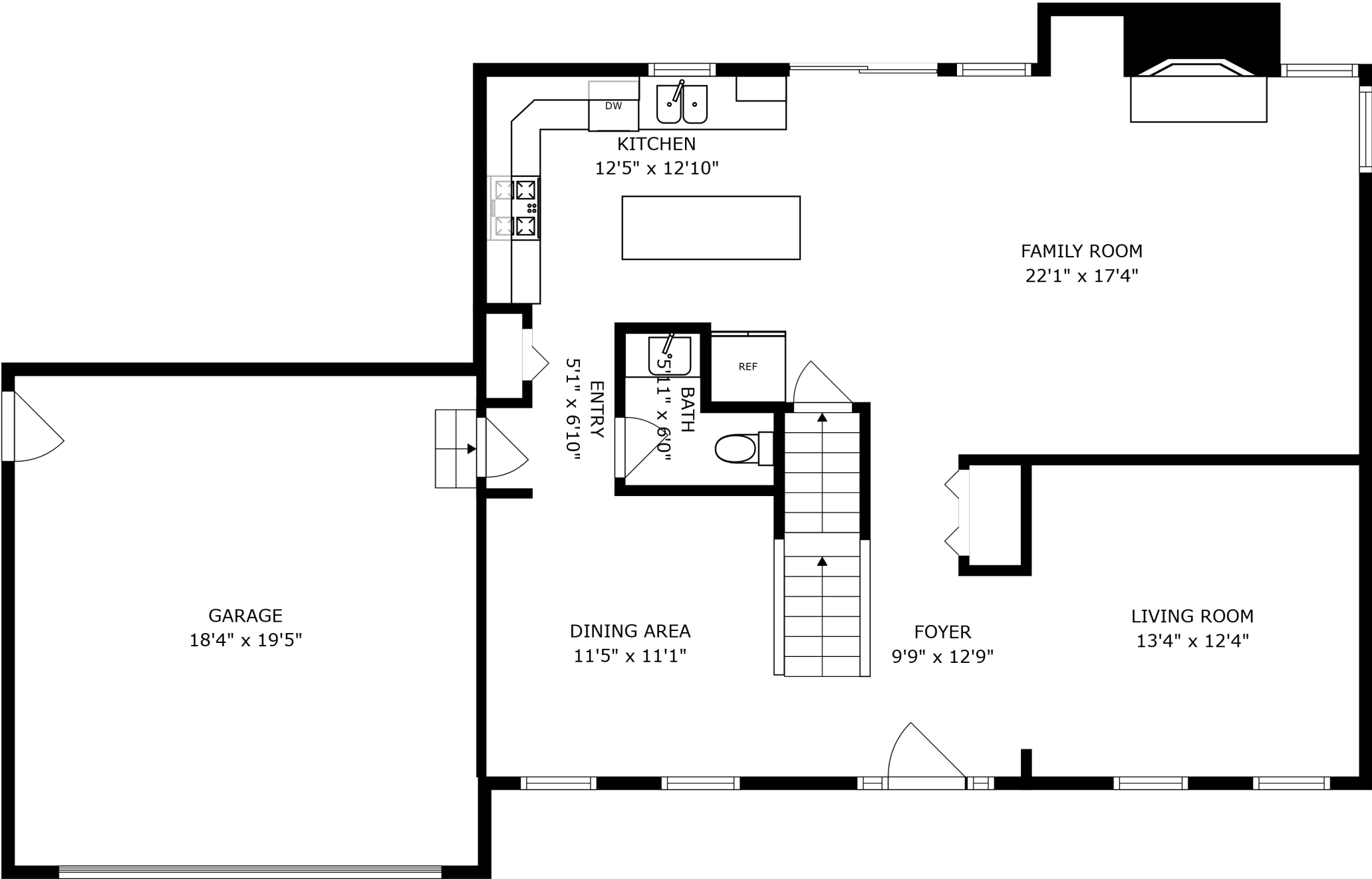
FLOOR 2
