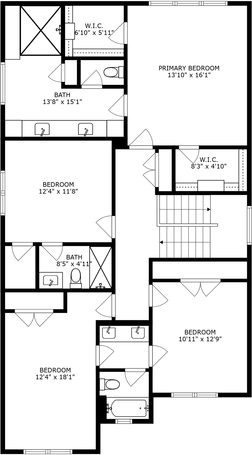
FLOOR 3
