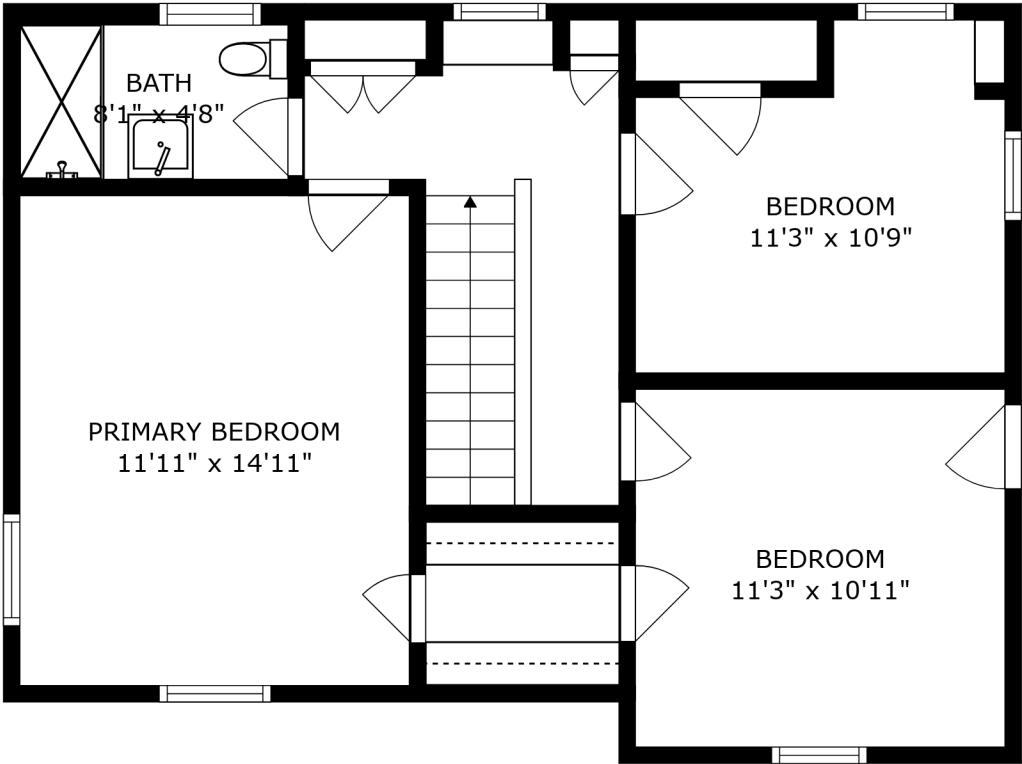
FLOOR 3
