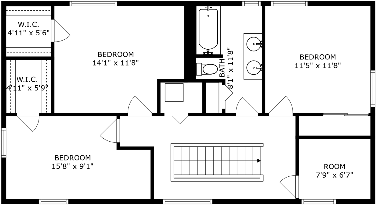
FLOOR 2
