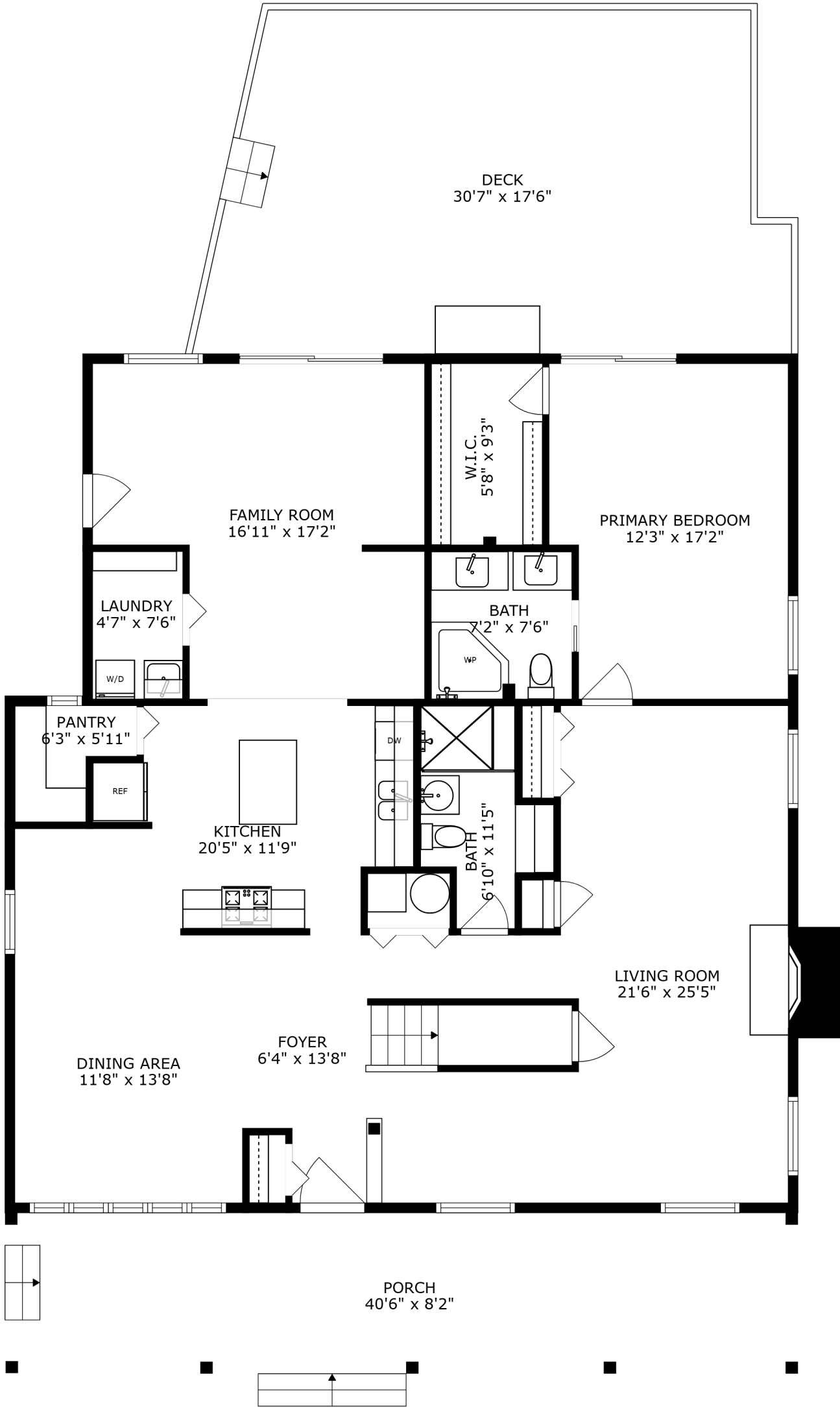
FLOOR 1
