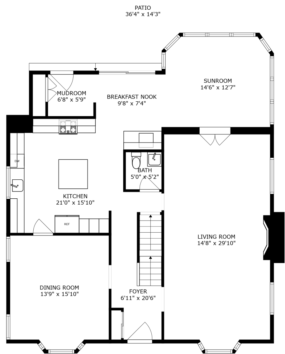
FLOOR 2
