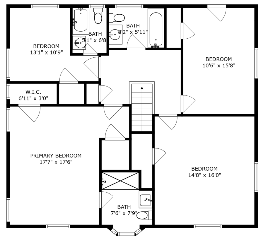
FLOOR 3
