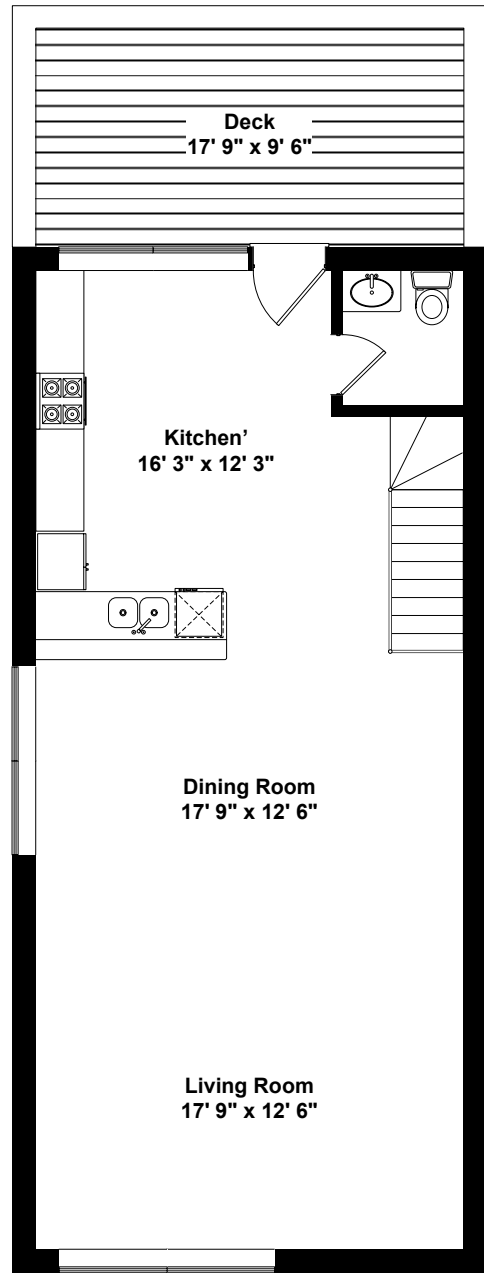
Third Floor
