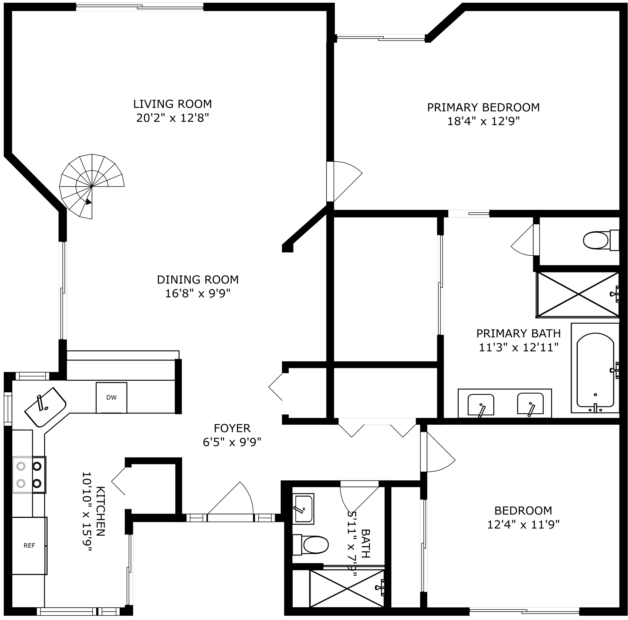
FLOOR 1
