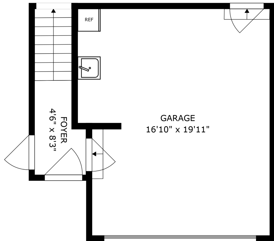
FLOOR 1
