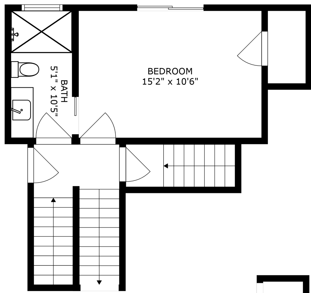
FLOOR 2
